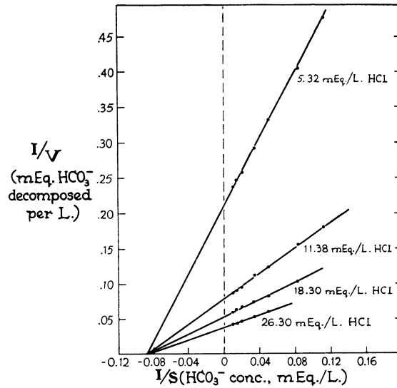
FIG. 5. RECIPROCAL PLOT OF BICARBONATE TITRATION EXPERIMENT
