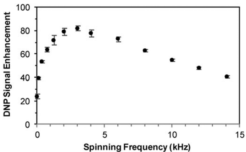
Fig. 10. Spinning frequency dependence of the ^1\text{H} DNP signal enhancement of 0.1 M \text{U-}^{13}\text{C-}^{15}\text{N} -proline in glycerol- \text{d}_8 - \text{D}_2\text{O} - \text{H}_2\text{O} (60 : 30 : 10 volume ratio), measured with ^{13}\text{C} CPMAS experiment at 97 K. Spectra were measured with and without microwave irradiation at each spinning frequency for calculation of the DNP signal enhancement. 10 s recycle delay, 1 dummy scan, 16 to 64 scans per experiment depending on the spinning frequency. Error bars are indicated on the plot.
