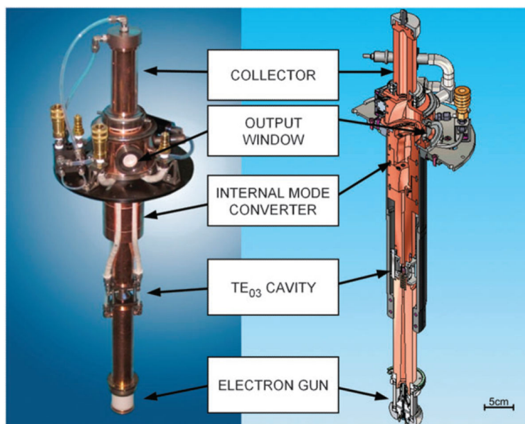
Fig. 1. Photograph and solid model cross section of 263 GHz gyrotron tube.
