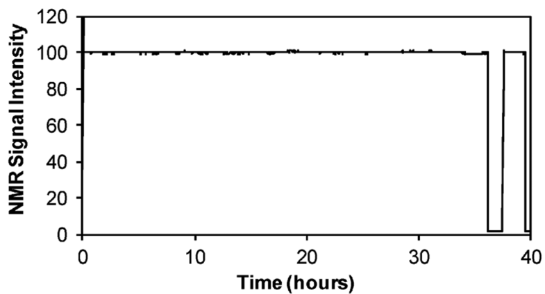
Fig. 11. NMR signal intensity for ^{13}\text{C}_\delta resonance of 0.1 M ^{13}\text{C} - ^{15}\text{N} proline in glycerol- d_8 - \text{D}_2\text{O} - \text{H}_2\text{O} (60 : 30 : 10 volume ratio) with 10 mM TOTAPOL during extended experiment run consisting of 36 h gyrotron-on, followed by 80 min gyrotron-off, 2 h gyrotron back on and off again. ^{13}\text{C} CPMAS experiment with 1.5 ms 55 kHz CP, 33 ms acquisition time with 100 kHz SPINAL64 decoupling, \omega_r/2\pi = 8 kHz, 97 K sample temperature, 16 scans, 1 dummy scan, 6 s recycle delay for each point.
