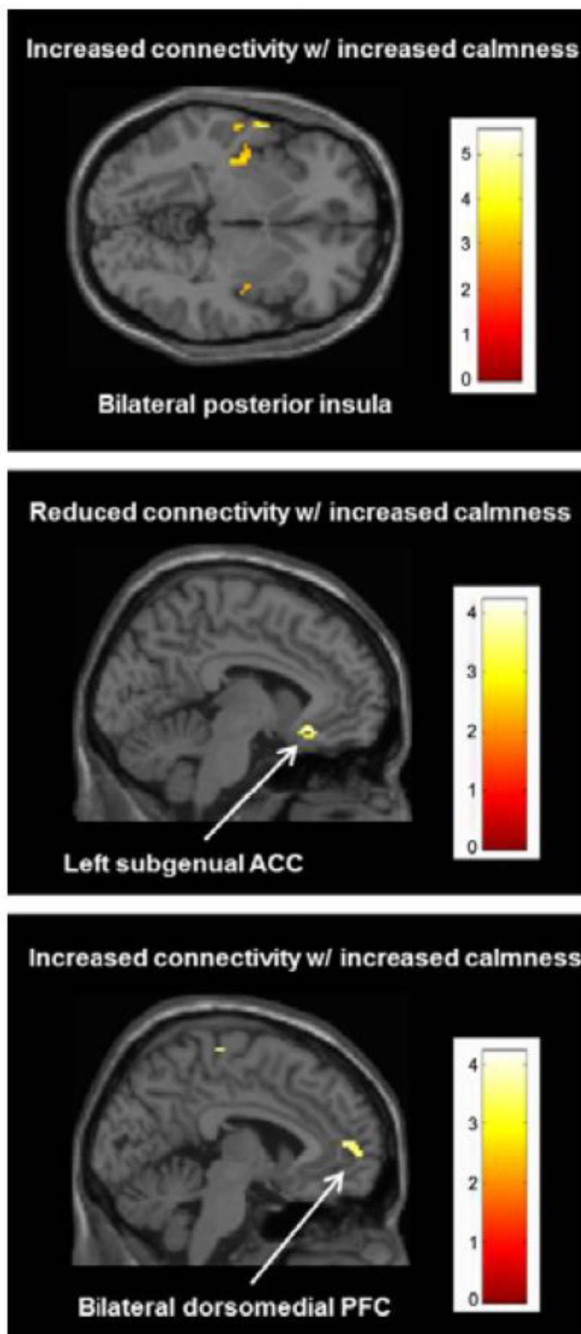
Fig. 3. Top panel: Clusters exhibiting a significant relationship between changes in calmness (Thayer subscale) and salience network connectivity ( P < 0.005 , corrected). Middle and bottom panels: Clusters exhibiting a significant relationship between changes in calmness (Thayer subscale) and default mode network connectivity ( P < 0.005 , corrected).
