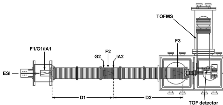
Figure 2. Schematic diagram of the IMS-MS instrument used in this study. Ion gates (G1 and G2), funnels (F1, F2, and F3), and activation regions (IA1 and IA2) are labeled. See text for details of instrument operation.
