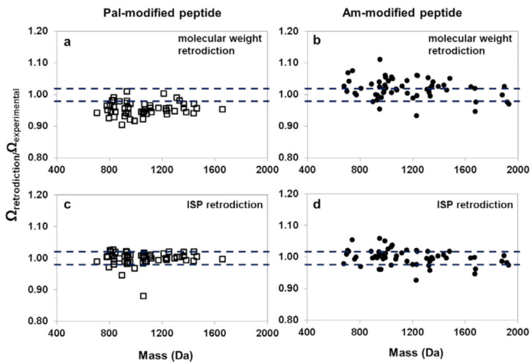
Figure 6. Prediction accuracy scatter plot for [\text{Pep}+2\text{H}]^{2+} ions modified with a Pal (empty squares) or an Am group (filled circles). Retrodictions are produced by a molecular weight fit for (a) Pal- and (b) Am-modified peptide ions (pentapeptides or longer). ISP retrodictions are displayed for these respective peptides in (c) and (d). Dotted lines indicate where the retrodicted values are within 2% of experimental values.
