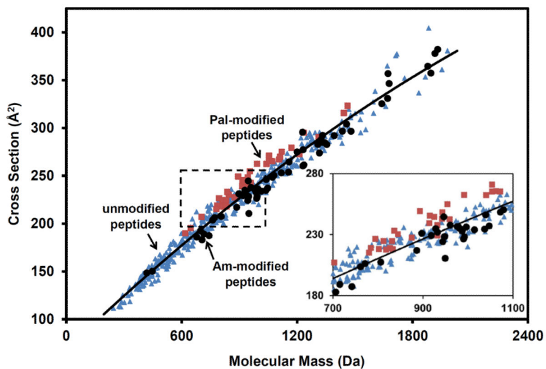
Figure 4. Cross sections as a function of molecular mass for [\text{Pep}+2\text{H}]^{2+} ions. The range of cross sections at a given molecular mass is displayed for [\text{Pep}+2\text{H}]^{2+} ions that are Pal-modified (red squares), Am-modified (black circles) or absent a chemical modification (blue triangles). A second-order molecular weight fit for all peptide ions is displayed over the data (black line). The inset shows an expanded region (overlaid dashed black square) of this relation of cross section for a given molecular mass.
