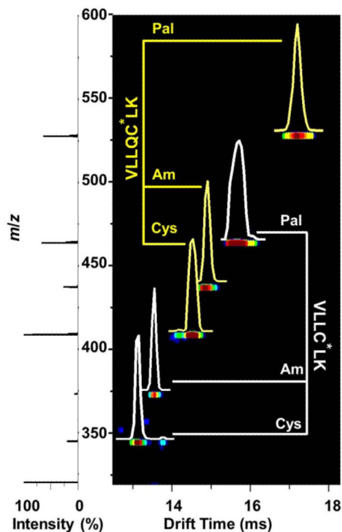
Figure 3. Nested IMS-MS dot plots of the electrosprayed mixture of two peptide sequences containing Cys, Cys Am , or Cys Pal residues. The sample concentration of each component is \sim 0.01 mg·mL -1 in 1:1 water:acetonitrile with 0.1% formic acid. The intensities of different features are represented using a false color scheme where the least intense features are shown in dark blue and the most intense are shown in red. The compressed mass spectrum displayed on the left is obtained by integrating across the entire range of m/z for each drift time. Drift time distributions are normalized to the peak height and overlaid for each peptide ion (VLLQC*LK and VLLC*LK are displayed in yellow and white, respectively). Within each sequence, C* annotates the modification site as the Cys residue. A branched scheme refers to peaks that correspond to each variable modification [unmodified (Cys) or modified with a carboxyamidomethyl (Am) or palmitoyl (Pal) group].
