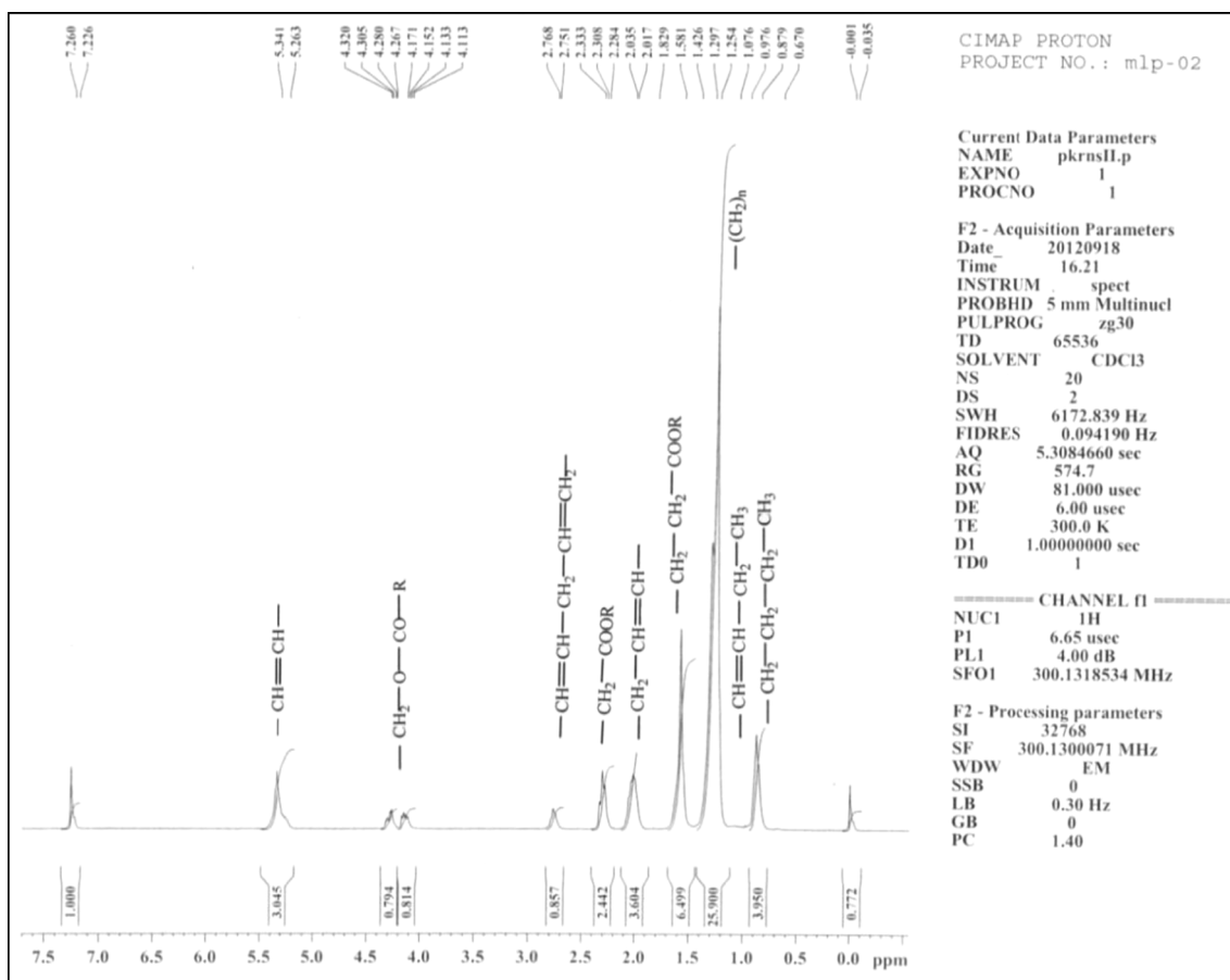
Fig. 3 ^1\text{H-NMR} spectrum of fatty oil
