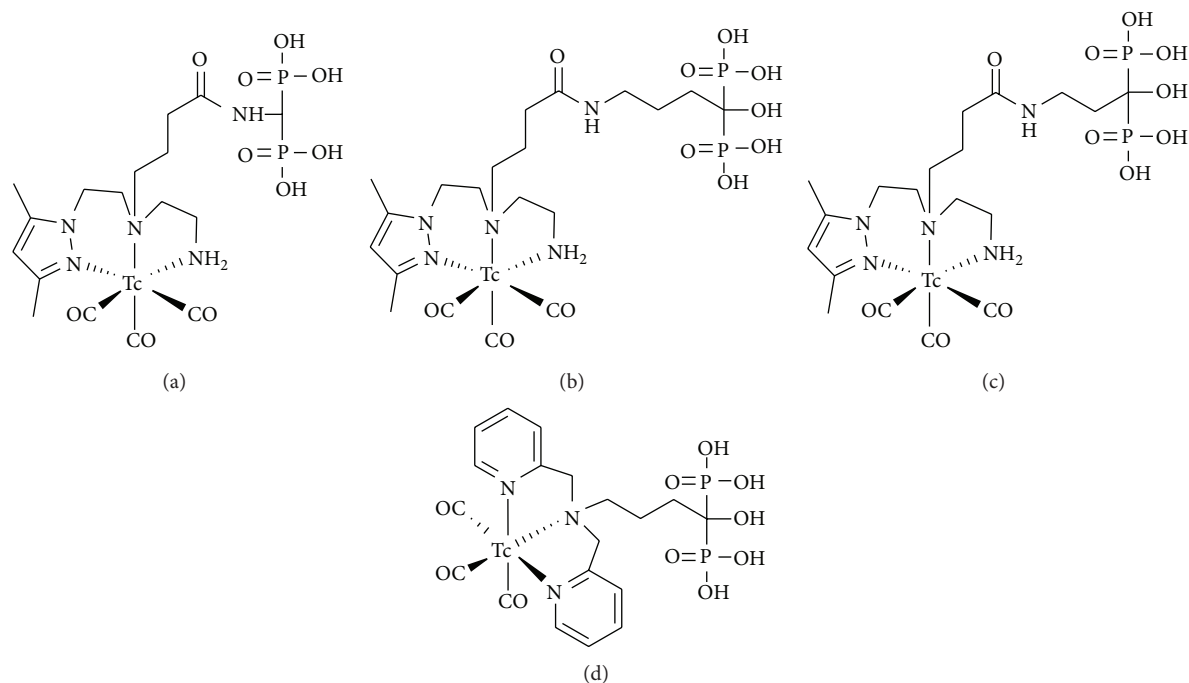
FIGURE 3: Chemical structures of ^{99m}\text{Tc} -tricarbonyl-complex-conjugated bisphosphonate compounds: (a) [^{99m}\text{Tc}(\text{CO})_3(\text{PzNN-BP})] , (b) [^{99m}\text{Tc}(\text{CO})_3(\text{PzNN-ALN})] , (c) [^{99m}\text{Tc}(\text{CO})_3(\text{PzNN-PAM})] , and (d) ^{99m}\text{Tc}(\text{CO})_3\text{-DPA-alendronate} .
