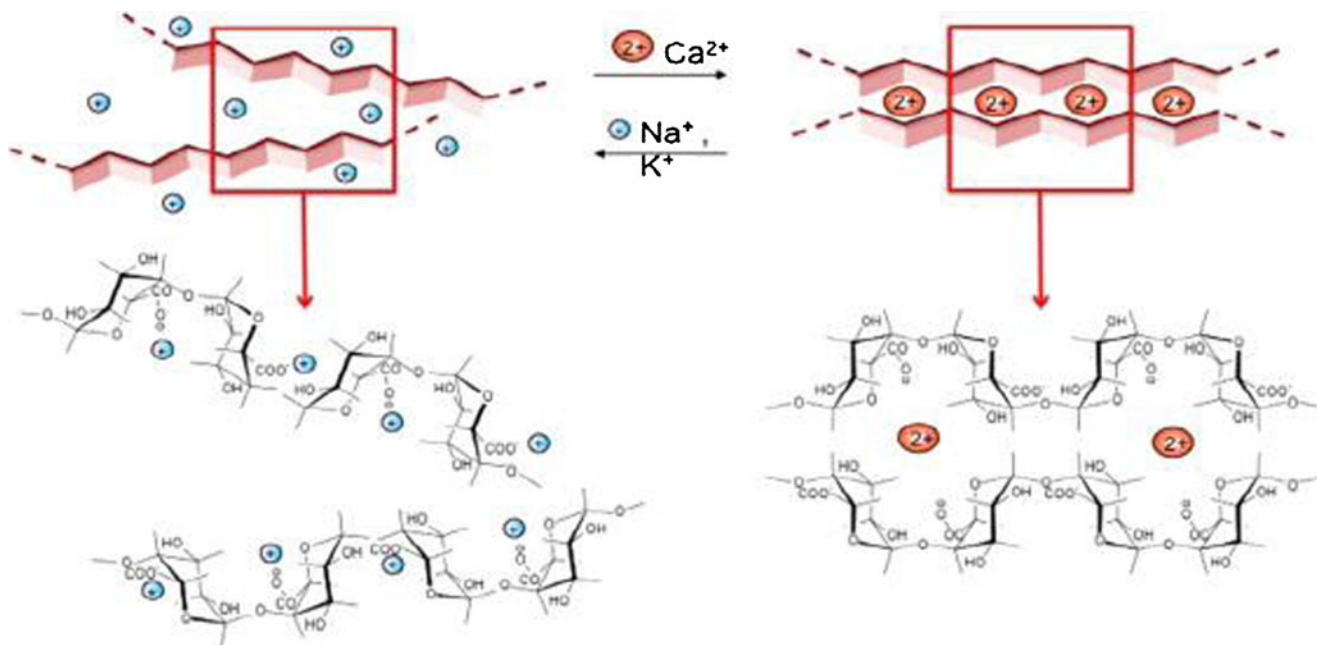
Fig. 2 Flow chart of preparation of pectin nanoparticles. Ca 2+ cross-links in a co-operating binding fashion between carboxylate group of adjacent chains enabling nanoparticle formation
