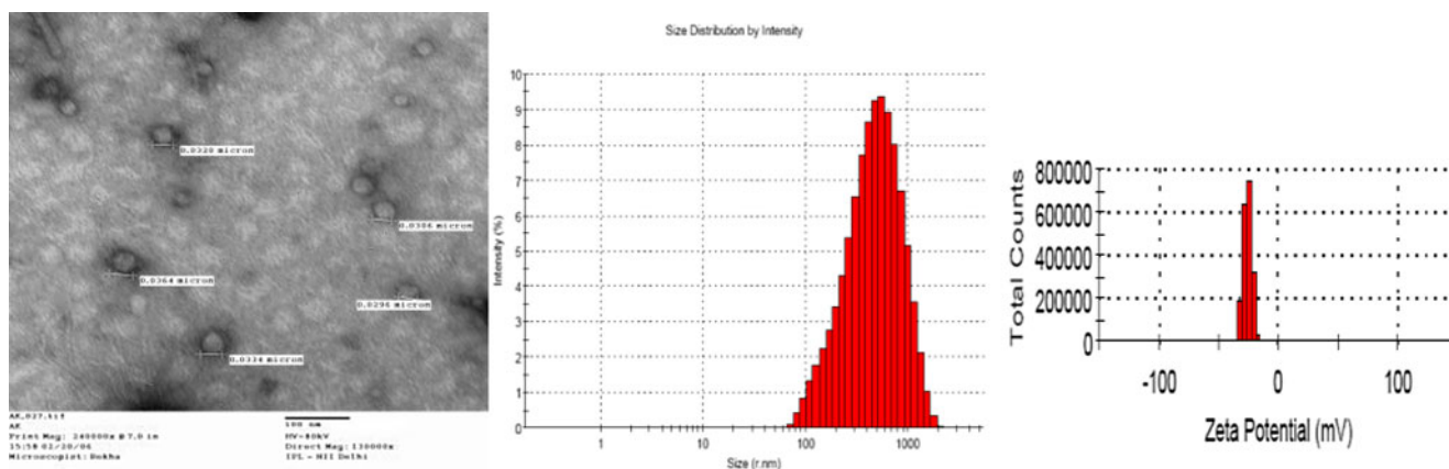
Fig. 1 TEM image of pectin nanoparticles. A representative graph of the size distribution spectra (~350 nm with PDI=0.30) and zeta potential (-26 mv)
