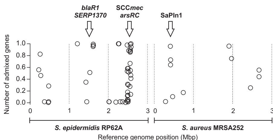
FIG. 5. —Genomic position of recombinated accessory genes in S. aureus and S. epidermidis based upon single-gene phylogenies. The frequency of admixed genes for 62 accessory genes with mixed ancestry phylogenies mapped to the corresponding locus in the reference S. epidermidis (RP62A) and S. aureus (MRSA252) genome. Example gene groups with high levels of interspecies gene flow are indicated.
