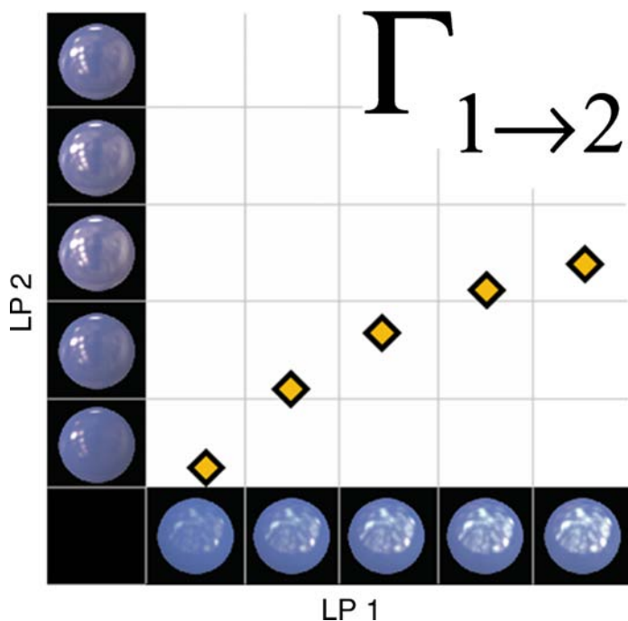
Figure 2. An illustration of the glossiness transfer function \Gamma for two light probes. Yellow diamonds represent points of perceived equal glossiness.
