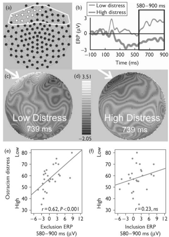
Fig. 2. Event-related potential (ERP) waveforms, and scalp topography of social exclusion and relations with distress. (a) Frontal electrodes correlated with ostracism distress during exclusion events for an ERP slow wave, highlighted in white (principal component analysis-derived slow wave, 580–900 ms, false discovery rate controlled). (b) ERPs for the average of electrodes in (a), 10 least versus 10 most distressed participants. (c) Interpolated voltage map for low distress group. (d) Interpolated voltage map for high distress group. (e) Scatter plot of mean slow wave data for exclusion events and ostracism distress scores ( n=27 ). (f) Scatter plot of mean slow wave data plotted for inclusion events during fair play and ostracism distress scores ( n=27 ).
