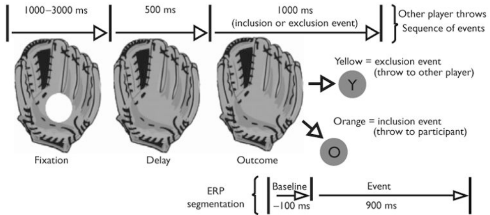
Fig. 1. Schematic diagram of a cyber-player's glove and events. The ball arrives at one of the cyber-player's gloves, remains for a fixation period, disappears (delay), and reappears as an outcome event (yellow ball for exclusion, orange ball for inclusion). Event-related potentials (ERPs) segmented on the outcome event.
