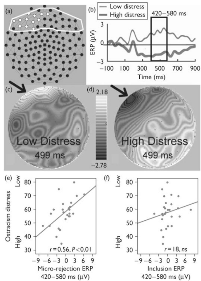
Fig. 3. Event-related potential (ERP) waveforms, and scalp topography of micro-rejection and relations with distress. (a) Frontal electrodes correlated with ostracism distress during micro-rejection events, highlighted in white (principal component analysis-derived window, 420–580 ms, false discovery rate controlled). (b) ERPs for the average of electrodes in (a), 10 least versus 10 most distressed participants. (c) Interpolated voltage map for low distress group. (d) Interpolated voltage map for high distress group. (e) Scatter plot of mean voltage data 420–580 ms for micro-rejection events and ostracism distress scores ( n=27 ). (f) Scatter plot of mean ERP voltage data plotted for inclusion events during fair play ( n=27 ).
