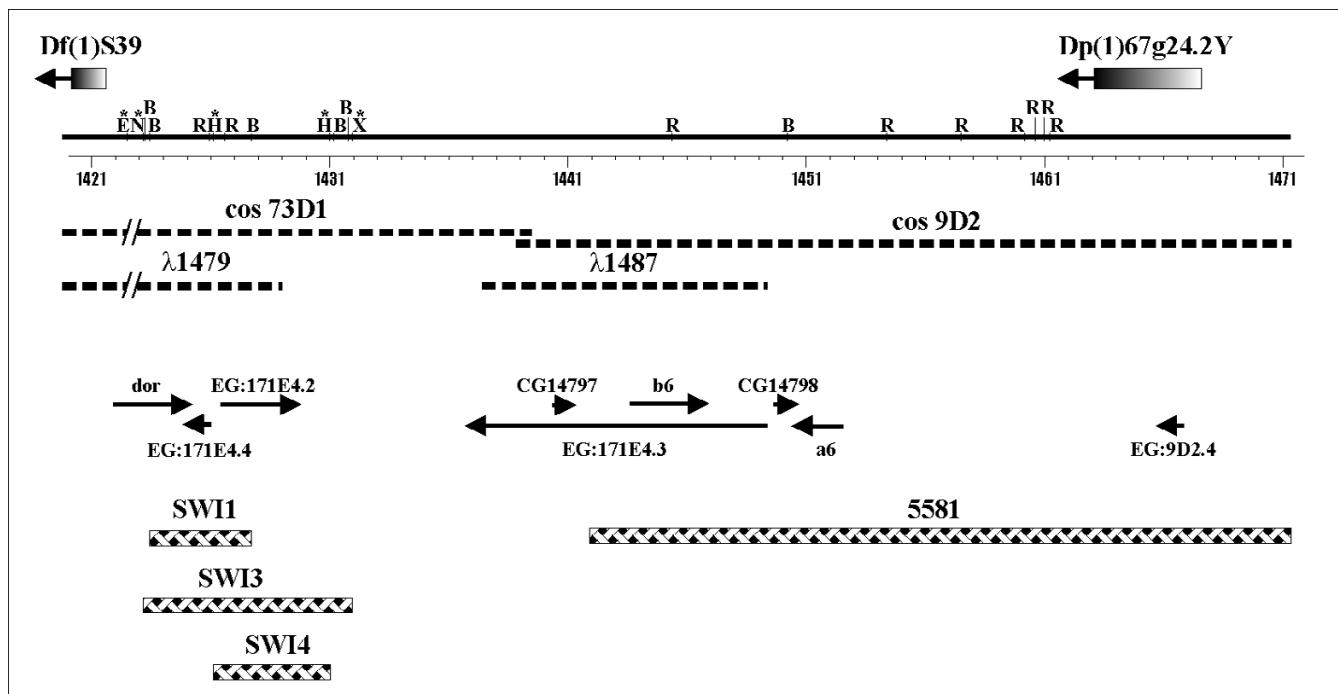
Figure 1 Organization of 2B6/B7-8 region The region is situated between the break points of Df(1)S39 and the duplication Dp(1;Y)y 267g24.2Y (shown by arrows). The shaded rectangles indicate the precision of rearrangement mapping. The restriction map of the region linked to the genomic sequence coordinates of FlyBase (in kb) is shown below. E-EagI , N-NheI , B-BamHI , X-XbaI , R-EcoR , H-HpaI . In the case of those sites marked with an asterisk only ones relevant to this study are shown. The positions of genomic clones (indicated by dashed lines), genetic loci (shown with arrows) and pieces of genomic DNA used for transformation (cross-hatched lines) are presented under the restriction map. The genes a6 and b6 correspond to CG3771 and CG3100 respectively.
