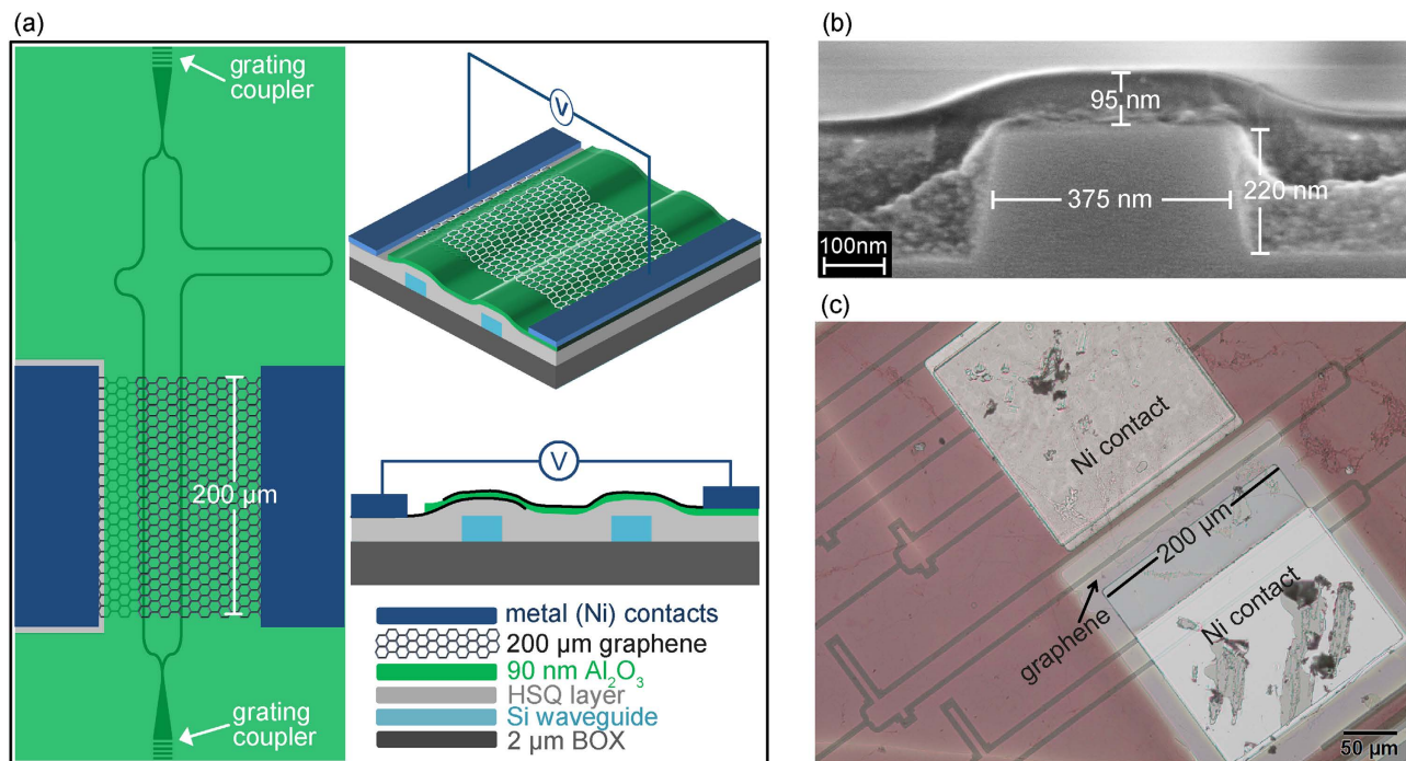
Figure 1. Graphene based electro-refractive phase modulator. (a) Schematic of the MZI used for determining \Delta n . Final layer of 40 nm \text{Al}_2\text{O}_3 is not shown for clarity. (b) Cross-section SEM image showing 95 nm (85 nm HSQ + 10 nm \text{Al}_2\text{O}_3 ) on top of MZI arm. (c) An optical image of final device.
