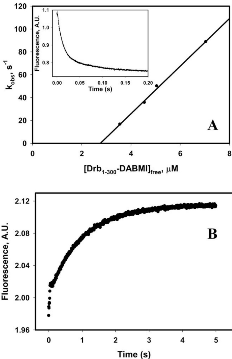
Fig. 4. Kinetics of Drb1-300 binding to actin filaments
