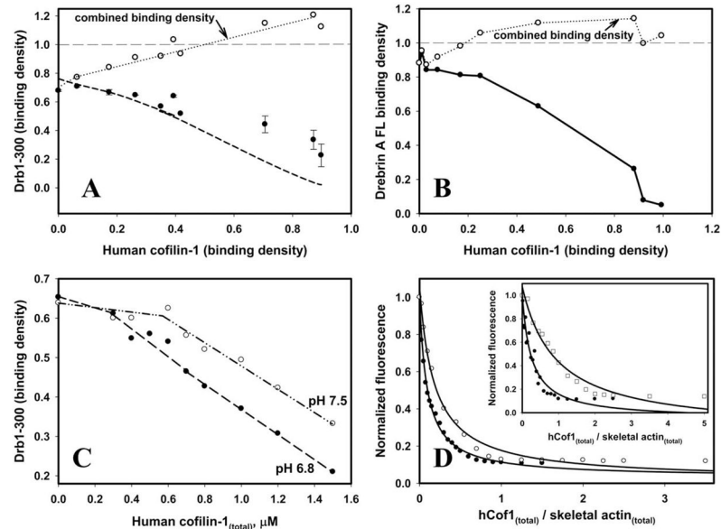
Fig. 3. Drebrin displacement from actin filaments by hCof1
