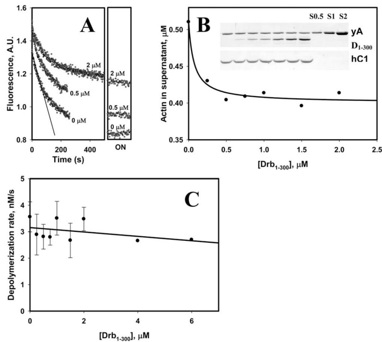
Fig. 2. Depolymerization of yeast WT F-actin in the presence of hCof1 and Drb1-300 (A) Examples of depolymerization data used to determine the initial rates of F-actin depolymerization. Depolymerization was followed by pyrene fluorescence. As an example, part of the data used to calculate the initial rate is indicated by a solid line. Fluorescence signals of the samples after overnight (ON) incubation, corrected for instrument-related drift of the signal, are shown in the right panel. Conditions: \text{KM}_2\text{EH}7.5 buffer supplemented with 1 mM DTT and 0.2 mM ATP. Final F-actin and cofilin concentrations were 2 and 1.5 \mu\text{M} , respectively. Concentrations of Drb1-300 in the samples are indicated next to the traces. (B) Drb1-300 decreases the extent of actin depolymerization in the presence of hCof1 compared to F-actin-cofilin control. Samples contain increasing concentrations of Drb1-300 (gel insert, left to right: 0; 0.25; 0.5; 0.75; 1; 1.5; 2 \mu\text{M} ). Conditions and protein concentrations as in (A.) Gel analysis (SDS PAGE, 12.5%) of the samples [as shown in (A)] after overnight incubation at 4°C. Supernatants and pellets were separated by high speed centrifugation and a representative gel of supernatant samples stained with Coomassie Blue is shown. Protein bands are marked as yA—yeast actin; D1–300—Drb1-300; hC1—human cofilin 1. Amounts of actin in supernatants were quantified using yeast actin standards (labeled as S0.5; S1; S2, numbers (0.5, 1, and 2) correspond to the actin concentration in \mu\text{M} ). Dependence of yeast WT F-actin (2 \mu\text{M} ) depolymerization rates in the presence of human cofilin-1 (1.5 \mu\text{M} ) on the concentration of Drb1-300 construct (average of two independent experiments). Conditions: 1\times \text{KM}_2\text{EH}7.5 buffer supplemented with 0.2 mM ATP and 1mM DTT.
