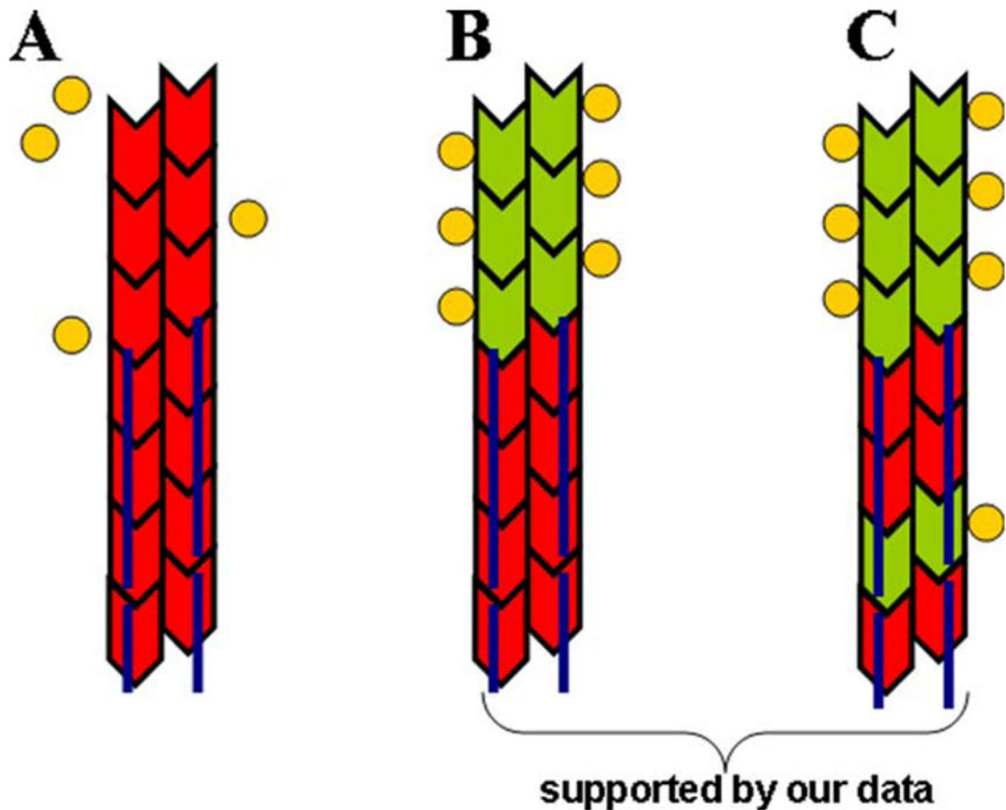
Fig. 6. Different scenarios of drebrin-cofilin competition for F-actin binding
