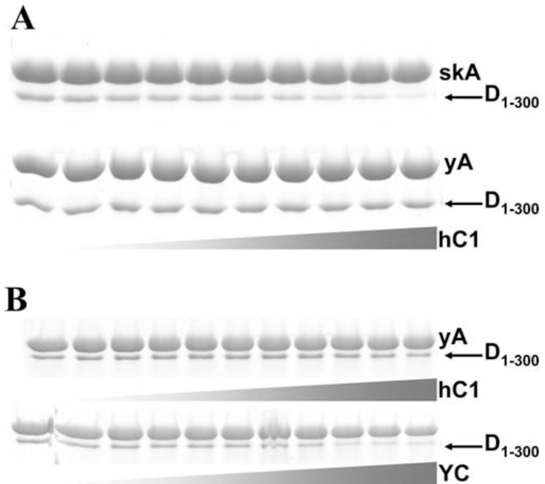
Fig. 5. Cofilin-mediated severing is a contributing factor in drebrin displacement from F-actin Gel analysis (SDS PAGE, 12.5%) of the samples. Supernatants and pellets were separated by high speed centrifugation. Representative gels stained with Coomassie Blue are shown (pellets only). (A) hCof1 at increasing concentrations (0.25; 0.4; 0.5; 0.6; 0.7; 0.8; 1; 1.5; 2; 2.5 \mu M) is added to 2 \mu M skeletal (top panel) or yeast F-actin (bottom panel) supplemented with Drb1-300 (1.5 \mu M); (B) hCof1 at increasing concentrations (0; 0.25; 0.4; 0.5; 0.6; 0.7; 0.8; 1; 1.5; 2; 2.5 \mu M) (top panel) or yeast cofilin (at the same concentrations as hCof1, bottom panel) is added to yeast F-actin (2 \mu M) supplemented with Drb1-300 (0.7 \mu M). Protein bands are labeled as follows: skA—rabbit skeletal actin; yA—yeast Saccharomyces cerevisiae actin; YC— Saccharomyces cerevisiae cofilin; hC1—human cofilin-1; D 1-300 —Drb1-300. Gray gradient-colored triangles represent schematically the range of increasing cofilin concentration (0–2.5 \mu M, from left to right). Conditions: 1 \times KM 2 EH7.5 buffer supplemented with 0.2 mM ATP and 1 mM DTT.
