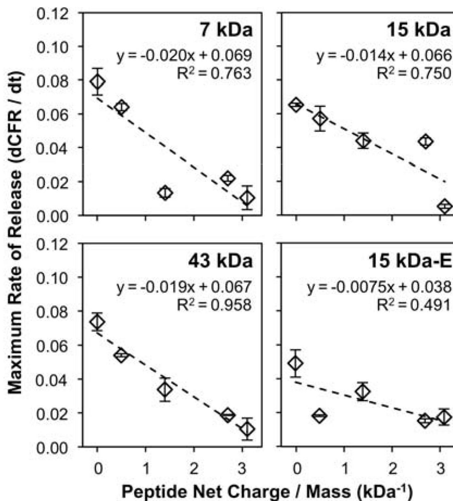
Fig 3. Release rates of peptides from PLGA MPs are inversely related to the peptides' net positive charge
