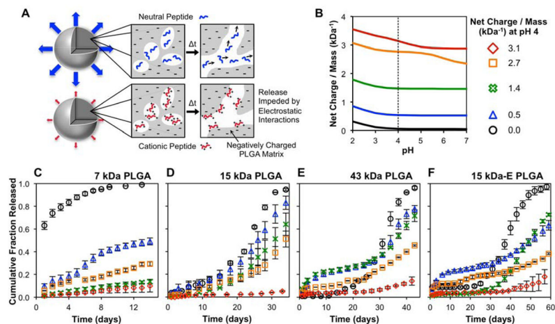
Fig 2. Greater net positive charge on a peptide corresponds with a reduction in release kinetics from negatively charged PLGA matrices
