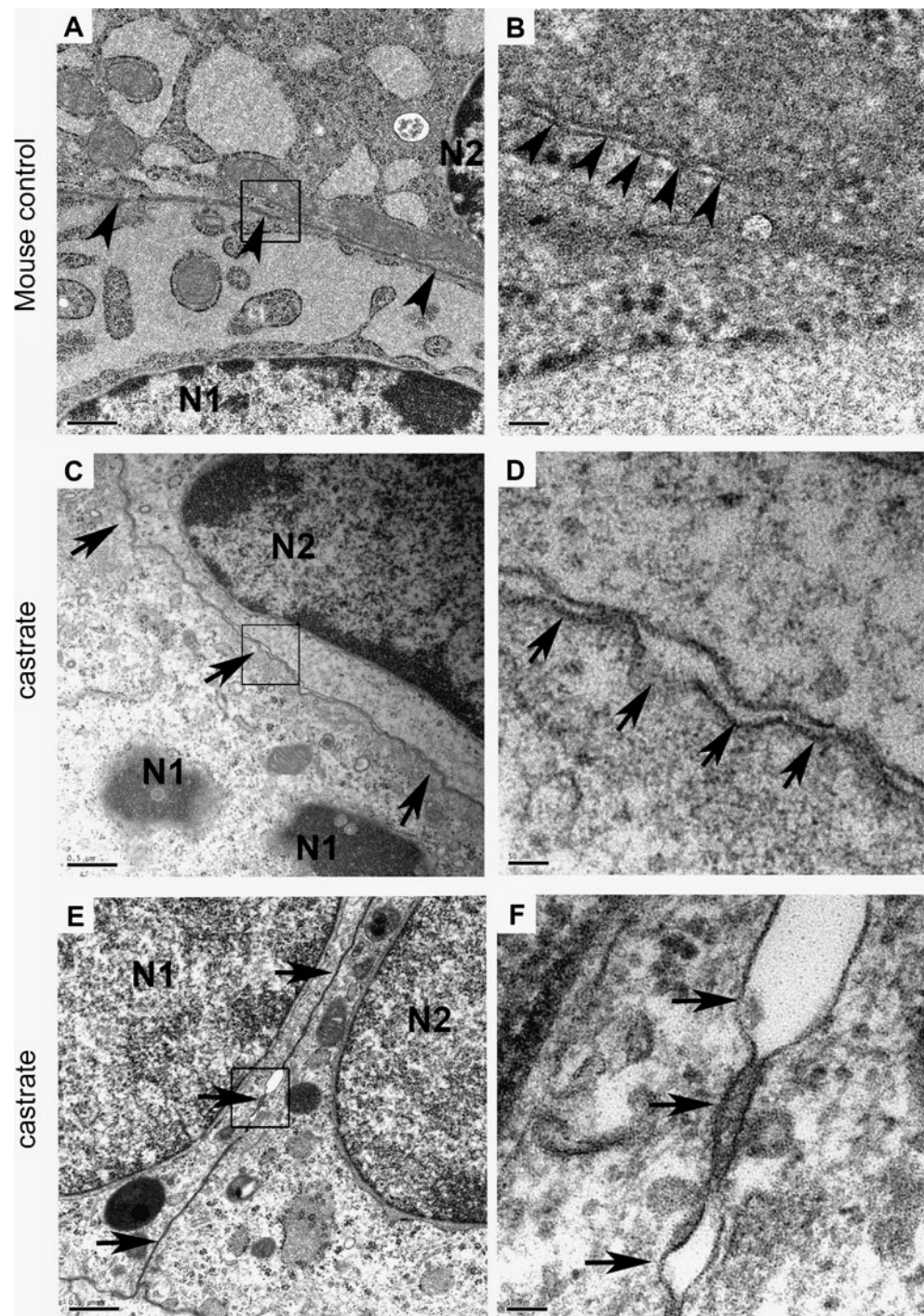
Fig. 2 Ultrastructure of prostate epithelium in normal and castrated mice. Normal epithelial tight junctions comprise a series of kissing points ( a, b ) (arrows) that juxtapose the lipid bilayers on opposing epithelial cells into intimate contact. In castrated mice, the tight junctions in the prostate epithelium lack obvious contact points ( c, d, e, f ), and the intercellular membranous contact regions are separated (arrows)
