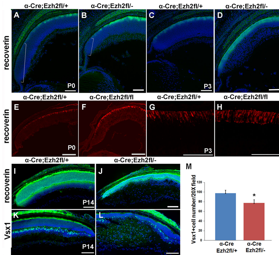
Figure 4. Ezh2 deletion increases rod photoreceptor differentiation in the early postnatal retina, and affects overall numbers of later born retinal cell types
