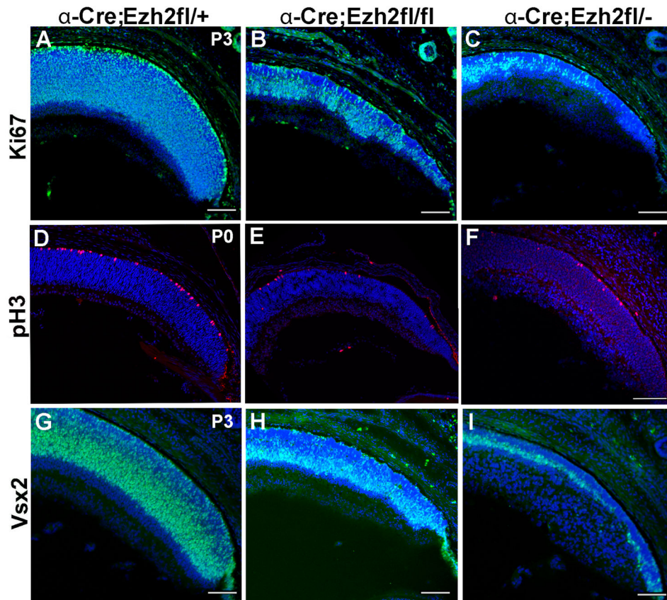
Figure 2. Ezh2 deletion results in reduced retinal progenitor proliferation
