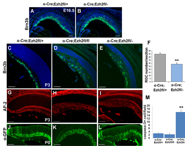
Figure 3. Ezh2 deletion alters retinal ganglion cell and amacrine cell numbers
