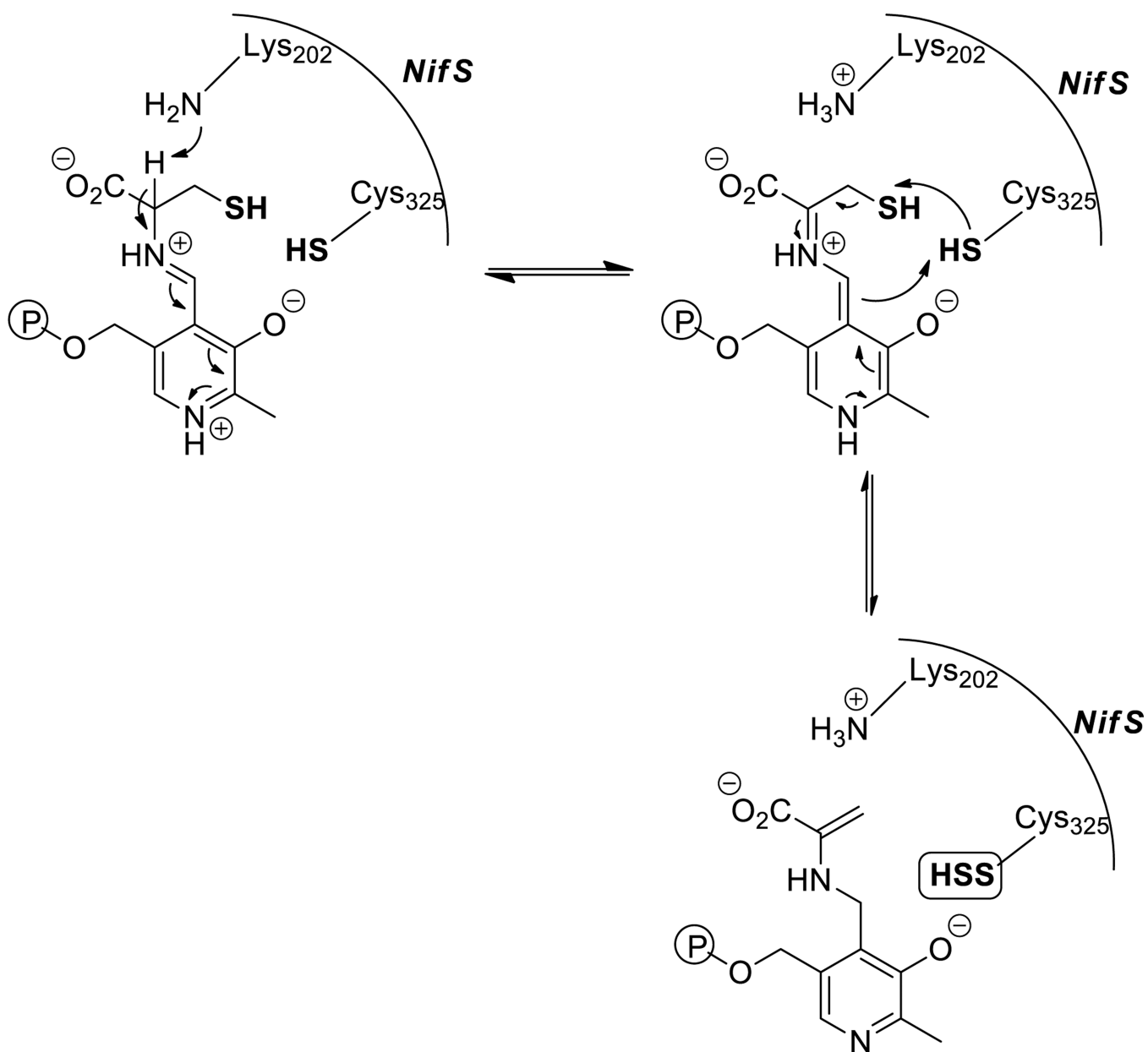
Scheme 12. Generation of NifS persulfide
