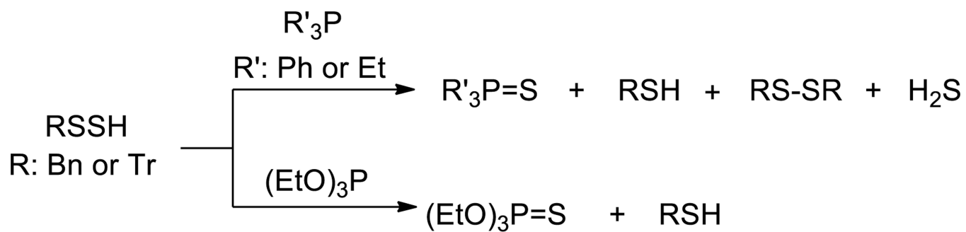
Scheme 6. Reactions of persulfides with phosphines and phosphites
