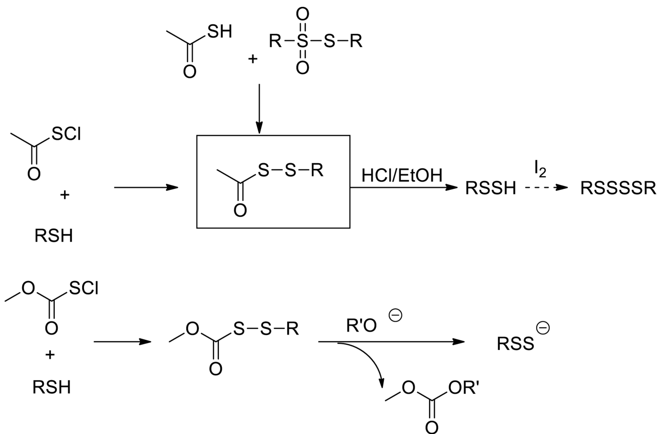
Scheme 2. Persulfide generation reactions
