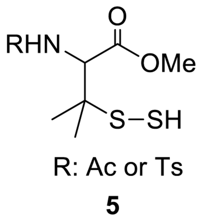
Scheme 3. Representative small molecule persulfides
