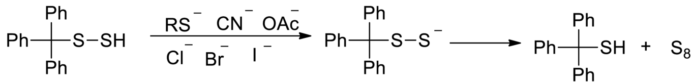
Scheme 7. Reactions of persulfides with various nucleophiles
