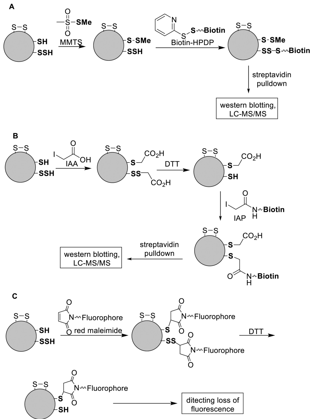
Scheme 17. Modified biotin switch assays for S-sulfhydration detection
