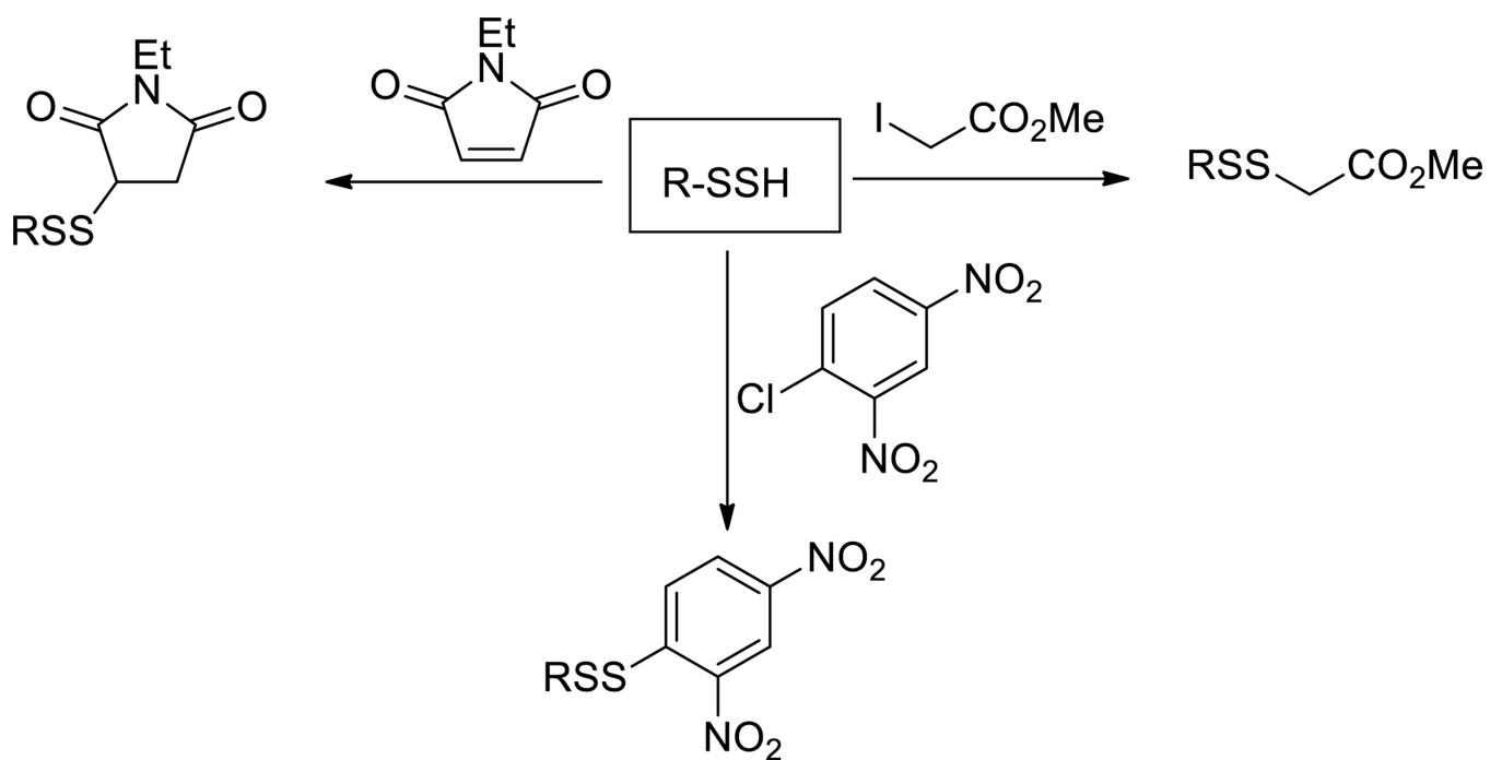
Scheme 8. Reactions of persulfides with selected electrophiles
