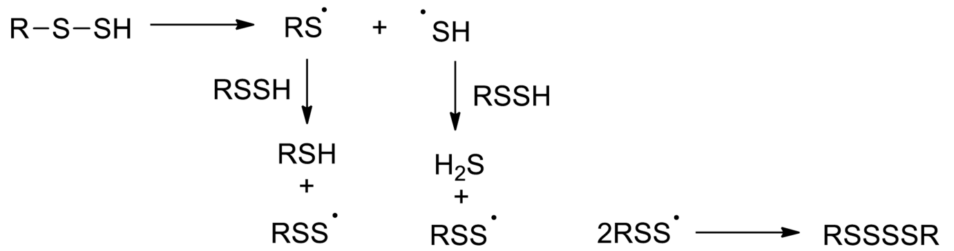
Scheme 5. Formation of perthiyl radicals
