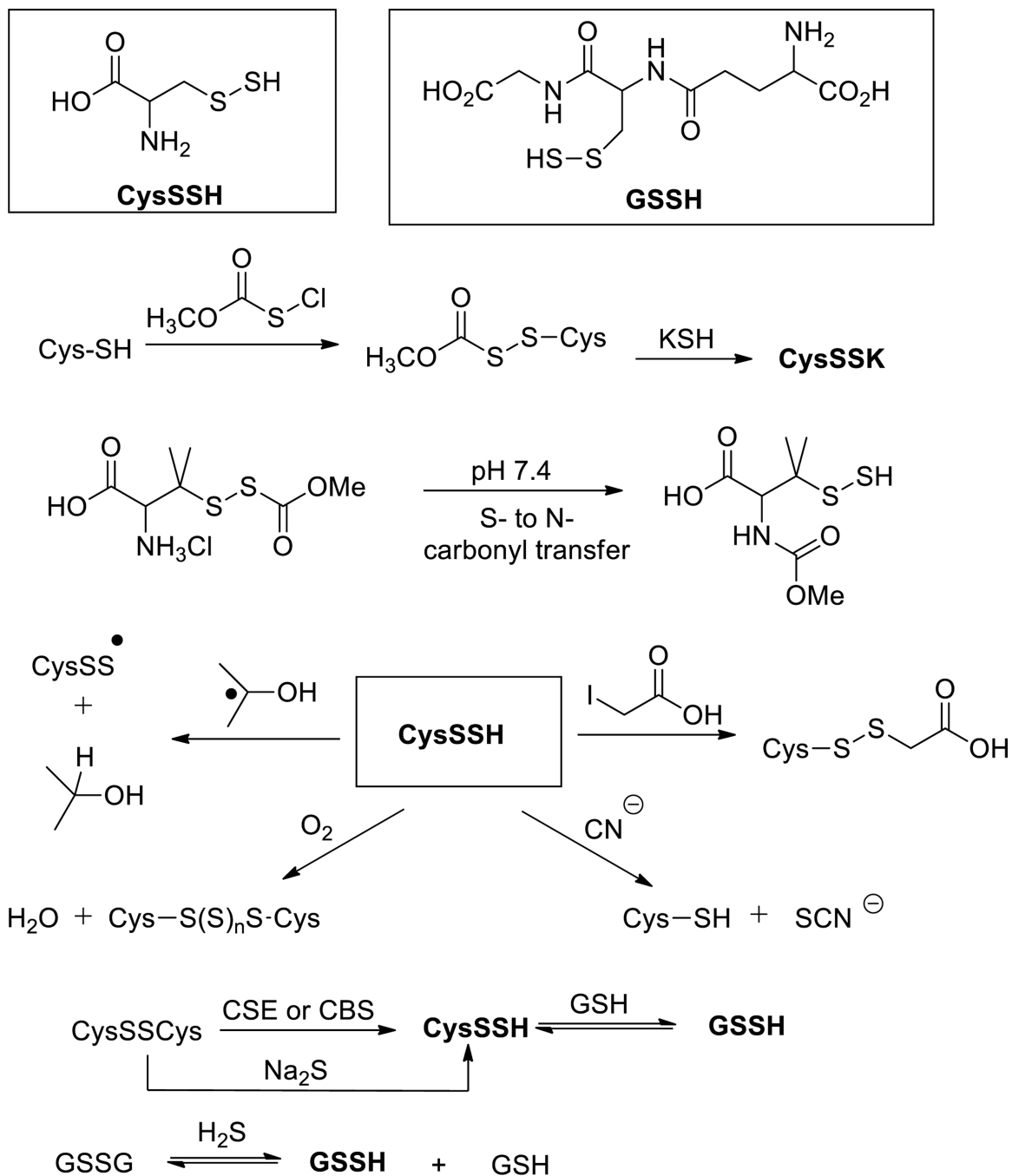
Scheme 11. Formation and reactivity of CysSSH and GSSH
