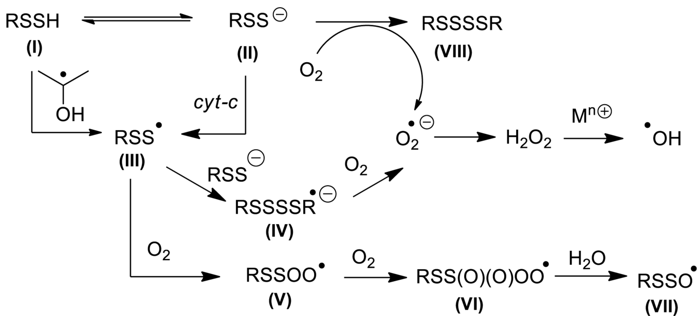
Scheme 10. Persulfides as pro-oxidants and antioxidants
