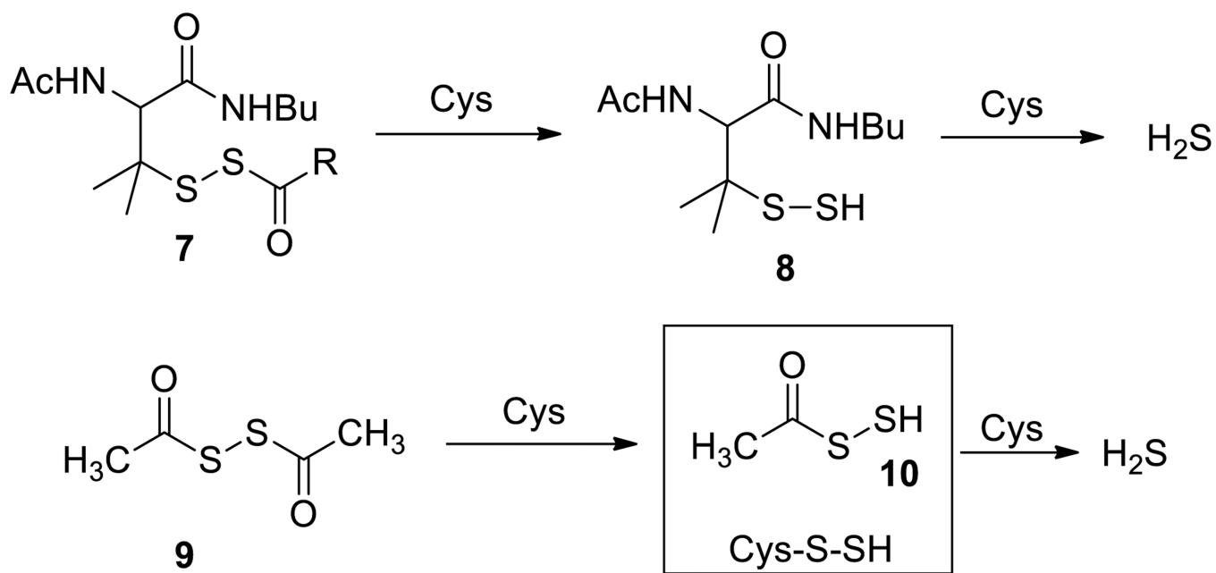
Scheme 4. Persulfide intermediates as H 2 S donors
