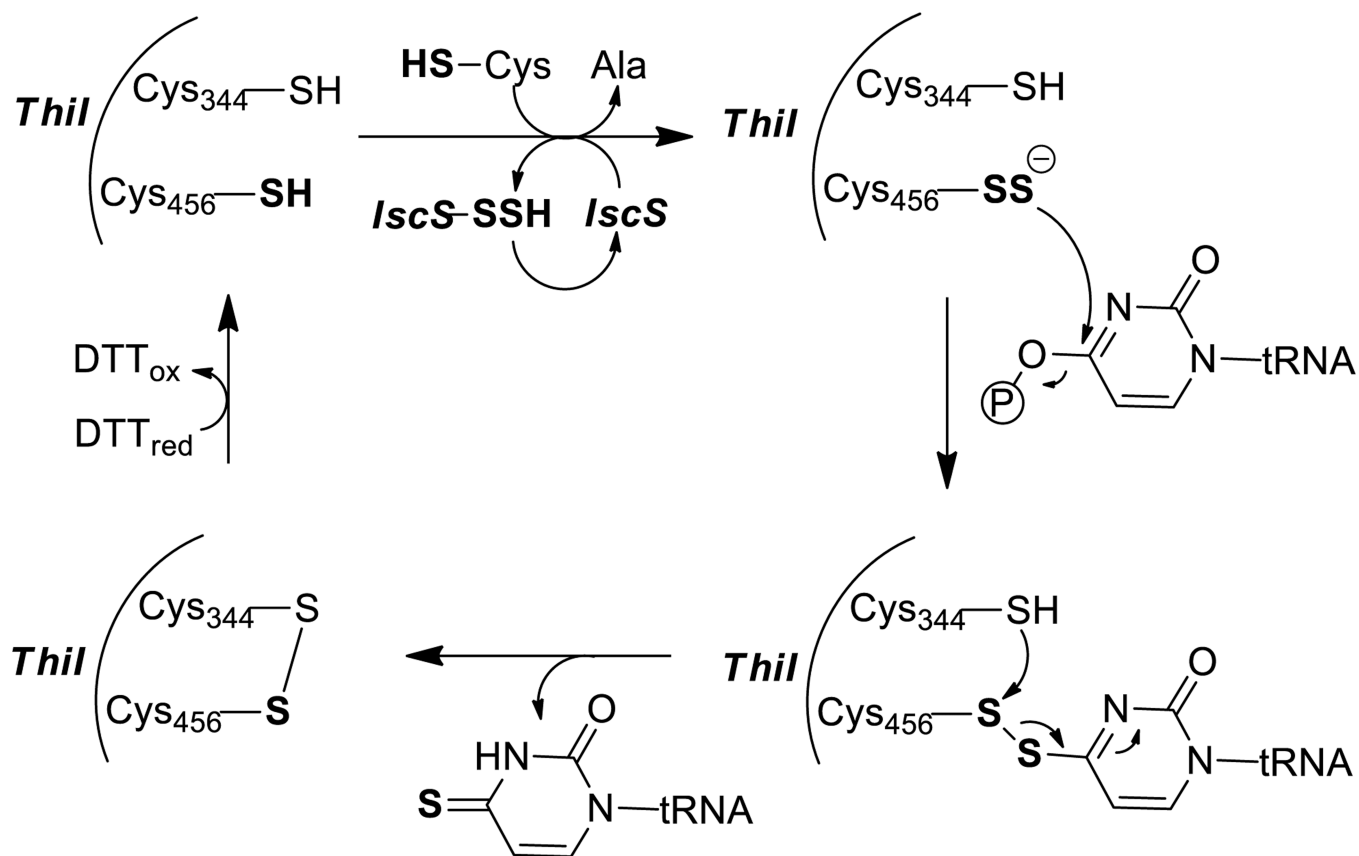
Scheme 13. Enzymatic formation of Thil persulfide and the sulphur transfer into tRNA
