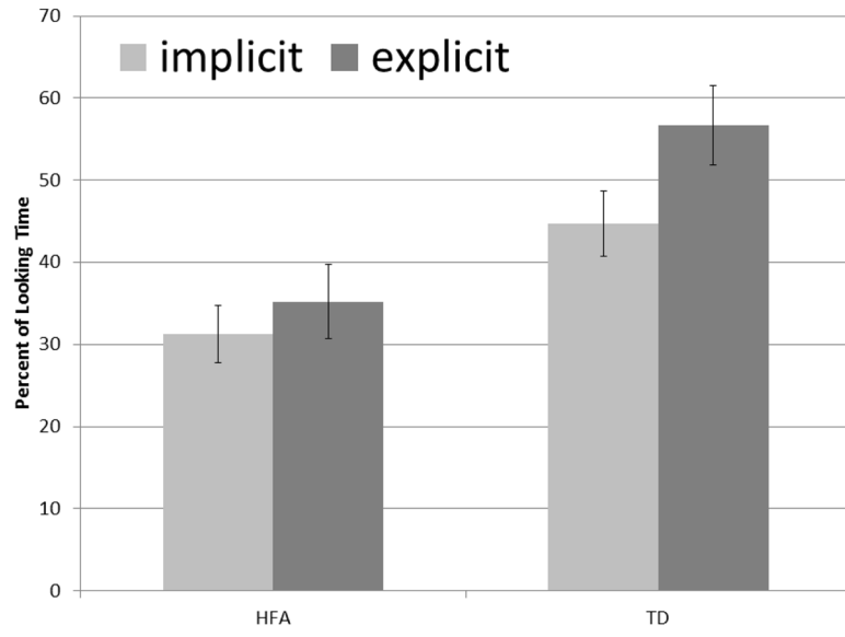
Figure 2. Percent Looking Time to In-Synch Video
