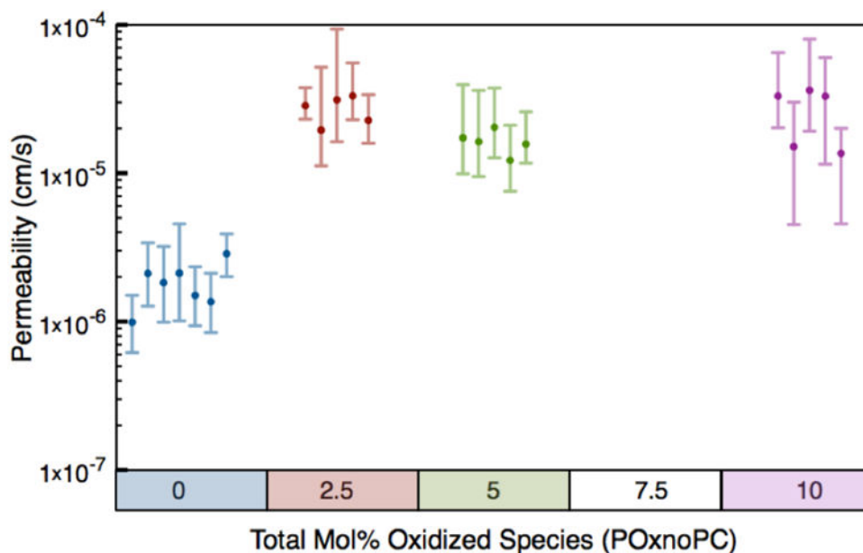
Figure 4. Measured permeability vs. percent oxidized species for four vesicle compositions. Each data point represents the calculated value and uncertainty for a single vesicle. Note that there appear to be two regimes of permeability: a slow regime for no POxnoPC present, and a fast regime for low levels (2.5–10%) POxnoPC present. The difference between these two regimes is over one order of magnitude.
