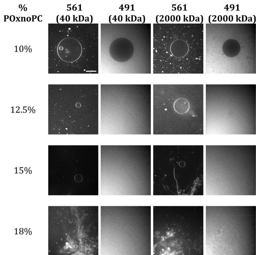
Figure 6. SDCM images showing pore formation for vesicles with 12.5–18% POxnoPC. The 10% POxnoPC images are shown as a reference for vesicles without pore formation, as neither species of fluorescein-dextran could enter the vesicle. For higher concentrations of oxidized species, both the 40 kDa and the 2000 kDa fluorescein-dextran was able to enter the vesicle. As both species are too large to enter the vesicle through passive transport pathways, this indicates that nanoscale pores are present in the membrane for these concentrations of oxidized lipid. Scale bar is 20 \mu\text{m} , and all images are the same resolution.
