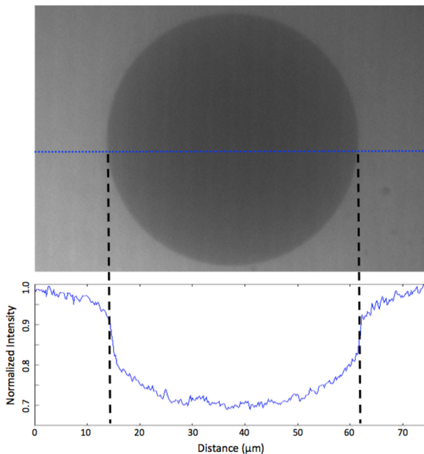
Figure 2. Intensity profile across a vesicle immersed in 1 mg/mL 40 kDa fluorescein-dextran. This image has been corrected for uneven illumination by flat-fielding. As the fluorescein-dextran cannot permeate the membrane, the intensity inside of the vesicle should be 0, and the profile across the vesicle should be flat. The presence of a non-flat profile indicates that there is pinhole crosstalk present in the experiments. This contribution to the intensity inside of the vesicle was accounted for during data analysis.
