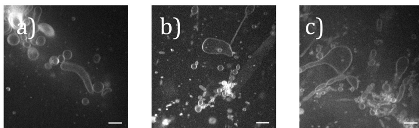
Figure 5. SDCM images showing vesicle formation for a) 12.5% POxnoPC, b) 15% POxnoPC, and c) 18% POxnoPC. For each composition, in addition to spherical vesicles, the lipids appear to form tubules and nonspherical structures. Spherical vesicles are typically quite small ( <10 \mu\text{m} in diameter). Scale bars are 10 \mu\text{m} .
