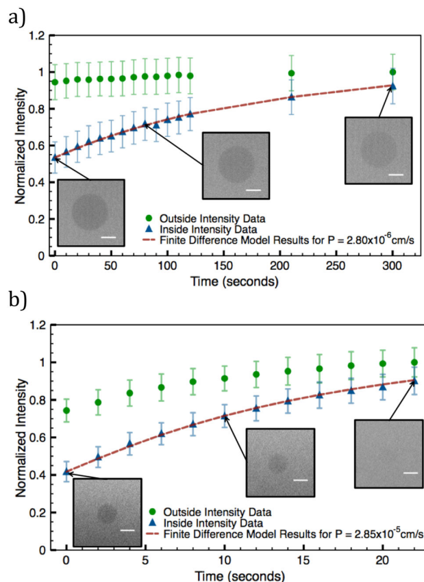
Figure 3. Intensity data and model fit for a data set with a) 0% POxnoPC and b) 2.5% POxnoPC. The green data points indicate the normalized outside intensity data (measured at one vesicle radius from the GUV membrane), the blue indicate normalized vesicle interior intensity data. The red line a) b) indicates the results of the finite difference model for the best-fit permeability. Image scale bars are 10 \mu\text{m} . The permeability of the 0% POxnoPC data in a) shows a permeability of 2.80 \times 10^{-6} cm/s, which is one order of magnitude lower than the permeability of the 2.5% POxnoPC membrane ( P = 2.85 \times 10^{-5} cm/s) shown in b).
