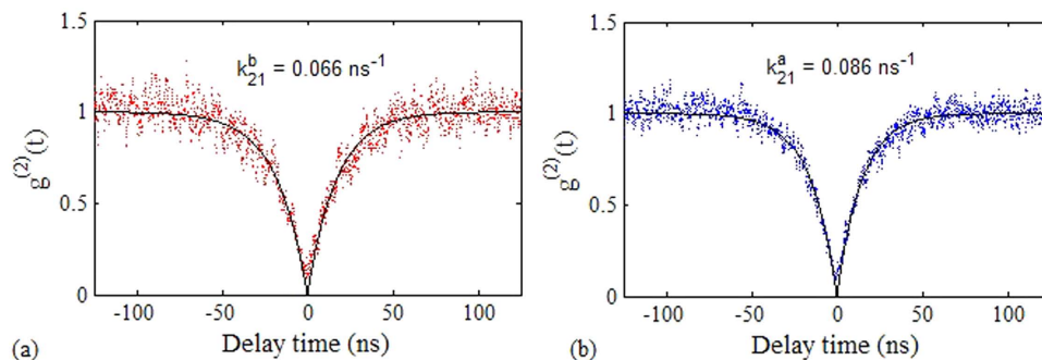
Figure 7. Intensity autocorrelation data as a function of delay time (a) before and (b) after PMMA coating with a time bin of 128 ps. The data was recorded at 50 \mu\text{W} pump power and fitted with a single exponential function (black curve), indicative of a two-level emitter. The calculated decay rates before and after coating are also provided.
