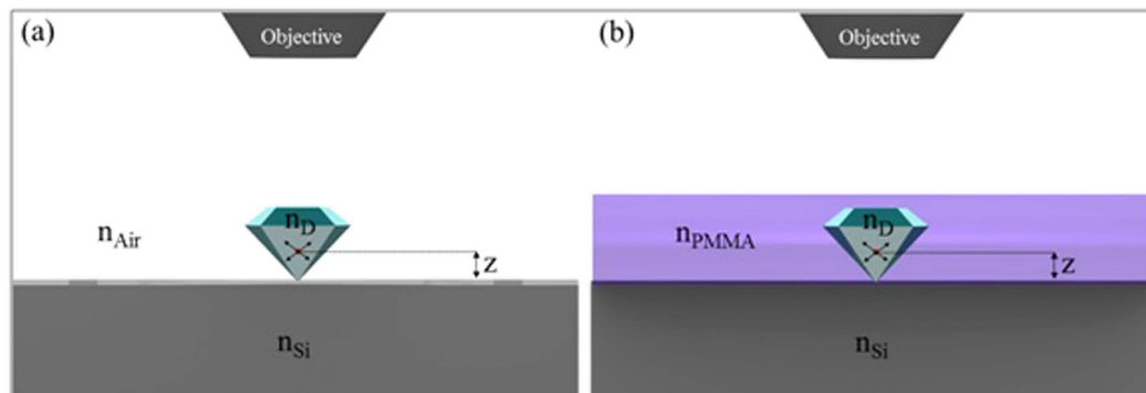
Figure 2. A simplified picture of the sample geometry, showing a single \text{NV}^- dipole enclosed in the ND, at a distance z from the lower ND-Si interface. The dipole's radiation was detected in the upper (a) ND/Air or (b) ND/PMMA interface with a 0.95NA objective lens.
