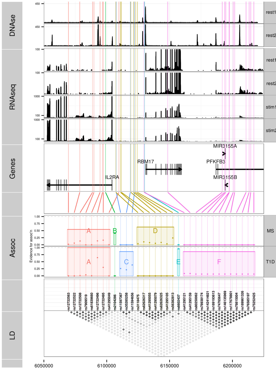
Fig 3. Six sets of SNPs can best explain the association of T1D and MS in the chromosome 10p15 region. LD: a heatmap indicating the r^2 between SNPs. Assoc: MPPI for MS and T1D are shown for the SNPs in a group, with total MPPI across a SNP group, gMPPI, indicated by the height of the shaded rectangle (see Table 5 for numerical details). SNP groups are labelled by the letters A-F for reference. SNPs in this track are ordered by SNP group for ease of visualisation. Genes: SNPs are mapped back to physical position and shown in relation to genes in the region. RNAseq: read counts in two pooled replicates of resting
