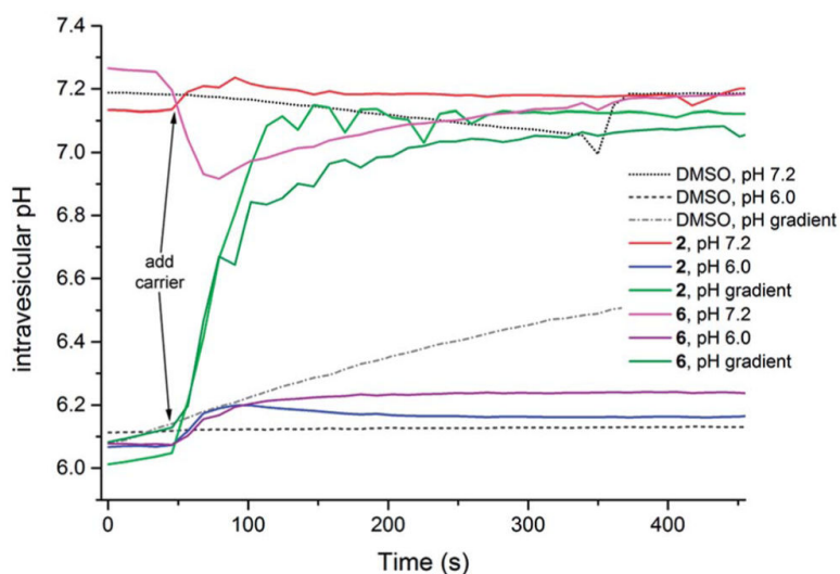
Fig. 6. Investigation of HCl transport facilitated by 1–8 using the fluorescent dye HPTS to estimate the intravesicular pH. For the experiments without pH gradient, POPC vesicles were loaded with 489 mM NaCl, 1 mM HPTS, buffered to pH 7.2 with phosphate buffer or to pH 6.0 with citrate buffer, and suspended in a solution of 489 mM NaNO 3 buffered to pH 7.2 with phosphate buffer or to pH 6.0 with citrate buffer. For the experiments with pH gradient, POPC vesicles were loaded with 489 mM NaCl, 1 mM HPTS, buffered to pH 6.0 with citrate buffer, and suspended in a solution of 489 mM NaNO 3 buffered to pH 6.0 with citrate buffer, and at time t = 0 s a NaOH solution was added to achieve an external pH of 7.0. At time t = 50 s a DMSO solution of the transporter was added (1 mol% with respect to lipid) and at time t = 350 s detergent was added. Each line represents the average of 3 independent trials and DMSO was used as a control.
