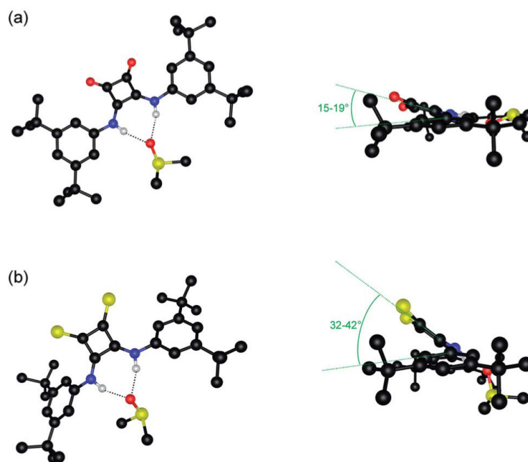
Fig. 1. Front and side views of the X-ray crystal structure of 4 -DMSO (a) and 8 -DMSO (b). Ligands and DMSO molecules are shown in ball-and-stick. Non-interacting hydrogen atoms and non-interacting DMSO molecules are omitted for clarity. Hydrogen bonds are represented by dashed lines and atoms are colour coded as follows: C (black), H (white), F (green), N (blue), S (yellow) and O (red). Relevant torsion angles are given in green.
