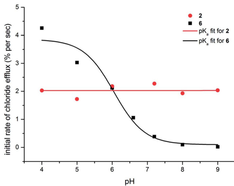
Fig. 7. pH dependence of the chloride transport ability of compounds 2 and 6 (1 mol% with respect to lipid). Chloride transport experiments were conducted as described in Fig. 5 but at various different pHs. The obtained data was fitted to an asymptotic function and the initial rate of chloride efflux was calculated (see ESI † for details) and plotted as a function of pH. Apparent pK_a values could subsequently be estimated by fitting the obtained plot to the following sigmoidal function: y = \max + ((\min - \max)/(1 + 10^{(pK_a - x)})) .
