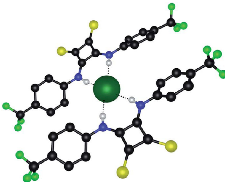
Fig. 3. X-ray crystal structure of 6 with TMA chloride. Ligands are shown in ball-and-stick and bound chloride is shown in spacefill (0.6 times van der Waals radius). TMA counterions and non-interacting hydrogen atoms are omitted for clarity. Hydrogen bonds are represented by dashed lines and atoms are colour coded as follows: C (black), H (white), F (green), N (blue), S (yellow) and Cl (dark green).
