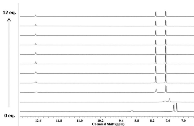
Fig. 2. Stack plot of the 1 H NMR spectrum of receptor 6 ( 2.5 \times 10^{-3} M) upon titration with chloride (0–12 eq.) added as its tertbutylammonium salt in CD 3 CN at 25 °C. From bottom to top: 0, 0.5, 1.0, 1.5, 2, 3, 4, 6, 8, 10, 12 equiv. chloride.
