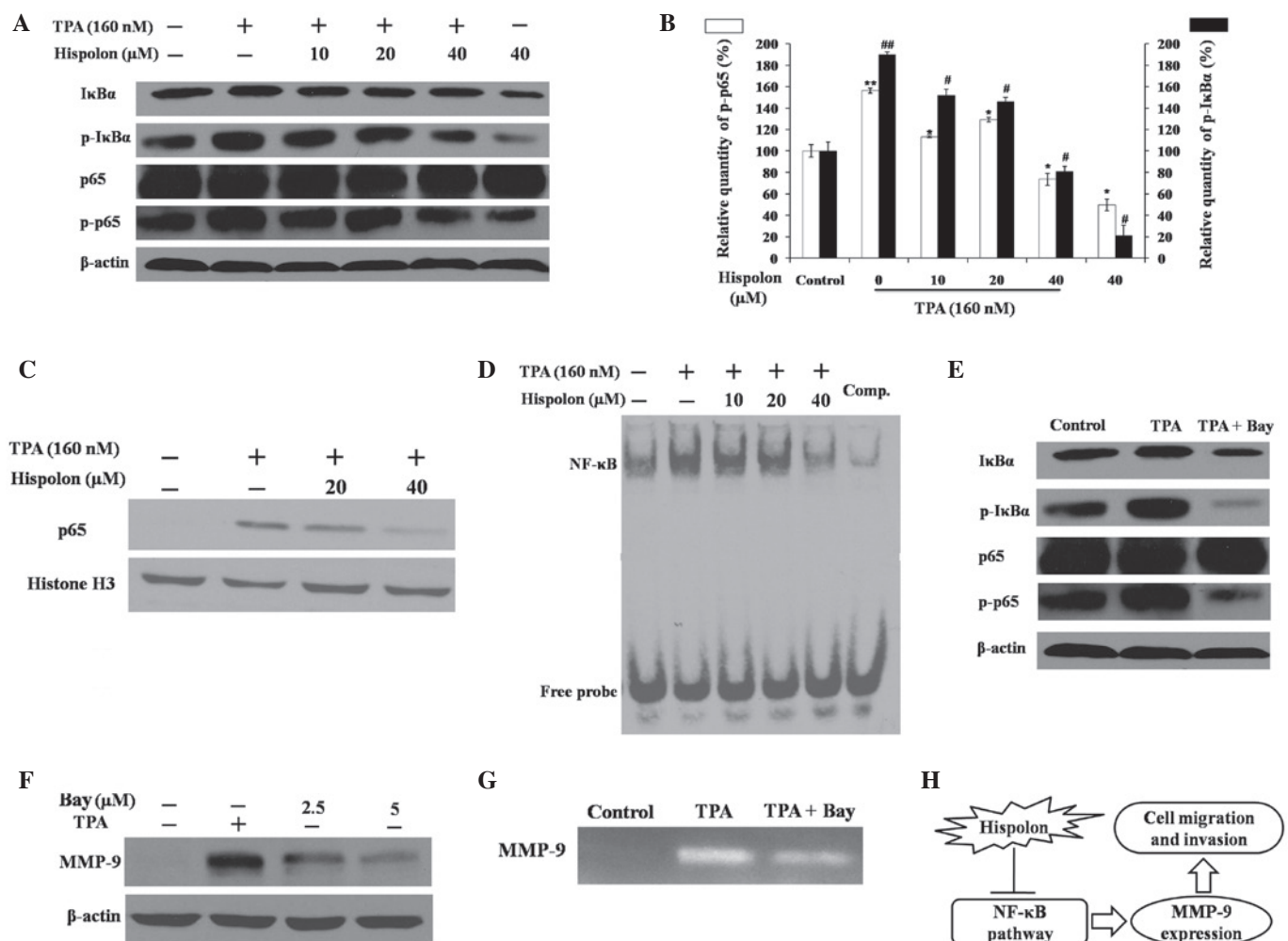
Figure 4. Hispilon inhibited the TPA-induced NF- \kappa B signaling pathway. (A) Hispilon inhibited the phosphorylation of I \kappa B \alpha and p65. Cells were pretreated with hispilon for 2 h prior to TPA incubation and then for another 2 h. Cell lysates were collected and subjected to western blot analysis for total I \kappa B \alpha , total p65, phospho-I \kappa B \alpha and phospho-p65 proteins. \beta -actin was used as an internal control. (B) Relative quantity of phosphorylated I \kappa B \alpha and p65 expression levels. * P <0.05 and # P <0.05 vs. TPA alone-treated group, ** P <0.05 and ## P <0.05 vs. DMSO control. All the data are presented as the mean \pm standard deviation of three independent experiments. (C) Hispilon prevented NF- \kappa B p65 nuclear translocation. Cells were preincubated with hispilon for 2 h prior to TPA treatment for another 2 h. Nuclear fractions were collected and histone H3 was used to verify equal loading. (D) Hispilon suppressed TPA-induced NF- \kappa B DNA-binding activity. MDA-MB-231 cells were treated as described in part (A). Nuclear extracts (10 \mu g) were incubated with biotin-labeled oligonucleotides containing the NF- \kappa B motif of the MMP-9 promoter. Bound mixtures were separated by 6% native-polyacrylamide electrophoresis. (E) Inhibitory effect of Bay 11-7082 on TPA-induced phosphorylations of I \kappa B \alpha and p65. Cells were pretreated with 5 \mu M Bay 11-7082 for 2 h and then stimulated with TPA for 2 h. (F) Inhibitory effect of Bay 11-7082 on TPA-induced MMP-9 expression. Cells in serum-free medium were pretreated with 2.5 or 5 \mu M Bay 11-7082 for 2 h and then stimulated with TPA for 24 h. Cell lysates were analyzed by western blot analysis. \beta -actin was used as an internal control. (G) Inhibitory effect of Bay 11-7082 on TPA-induced MMP-9 secretion. Cells in serum-free medium were preincubated with 5 \mu M Bay 11-7082 for 2 h, followed by treatment with TPA for 24 h. (H) Schematic diagram of the molecular mechanisms underlying the antimetastasis activity of hispilon in TPA-induced MDA-MB-231 cells. TPA, 12- O -tetradecanoylphorbol-13-acetate; DMSO, dimethyl sulfoxide; NF- \kappa B, nuclear factor- \kappa B; MMP-9, matrix metalloproteinase-9; Comp., competitor.
