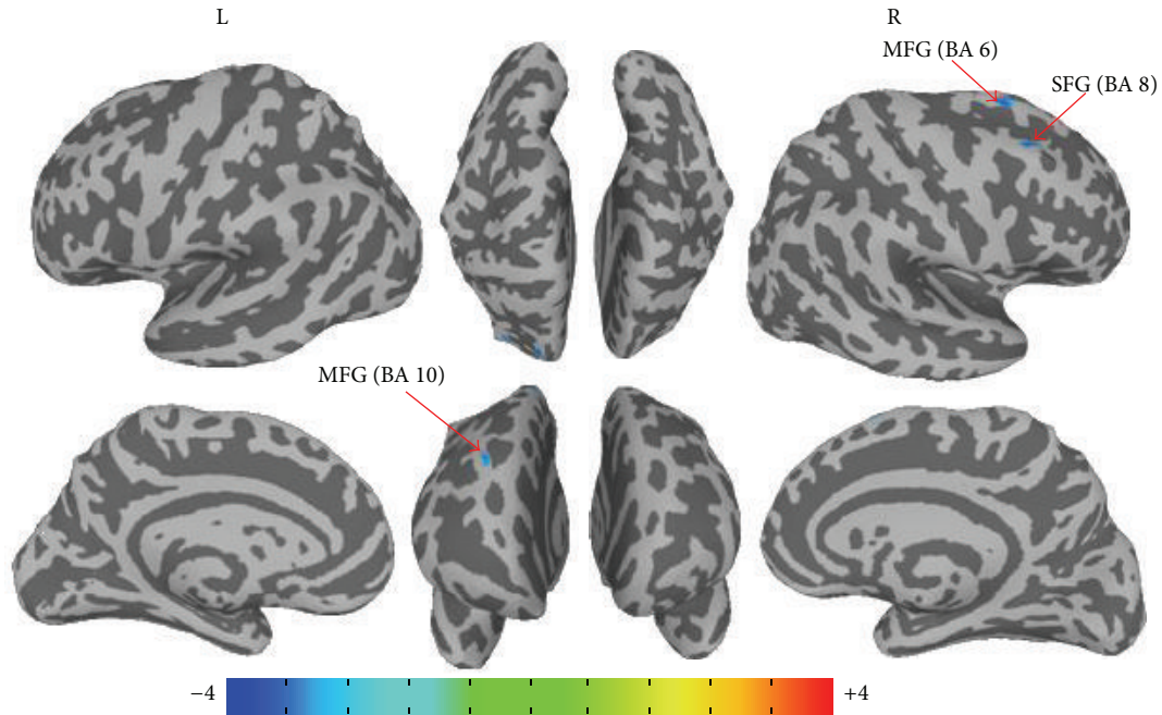
FIGURE 3: Changed functional connectivity of right ACC after acupuncture for patients with Bell's palsy at early stage. P \leq 0.01 , \alpha \leq 0.05 , corrected with Monte-Carlo method. BA: Brodmann area; SFG: superior frontal gyrus; MFG: right middle frontal gyrus; MFG: middle frontal gyrus.
