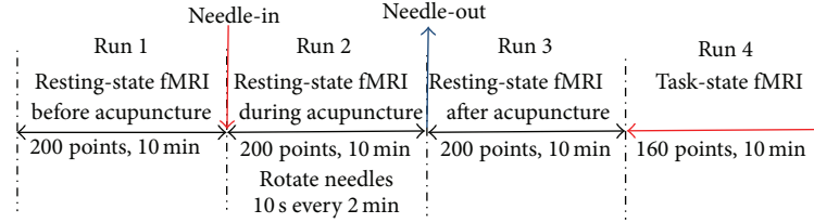
FIGURE 2: fMRI paradigms of the experiment.
