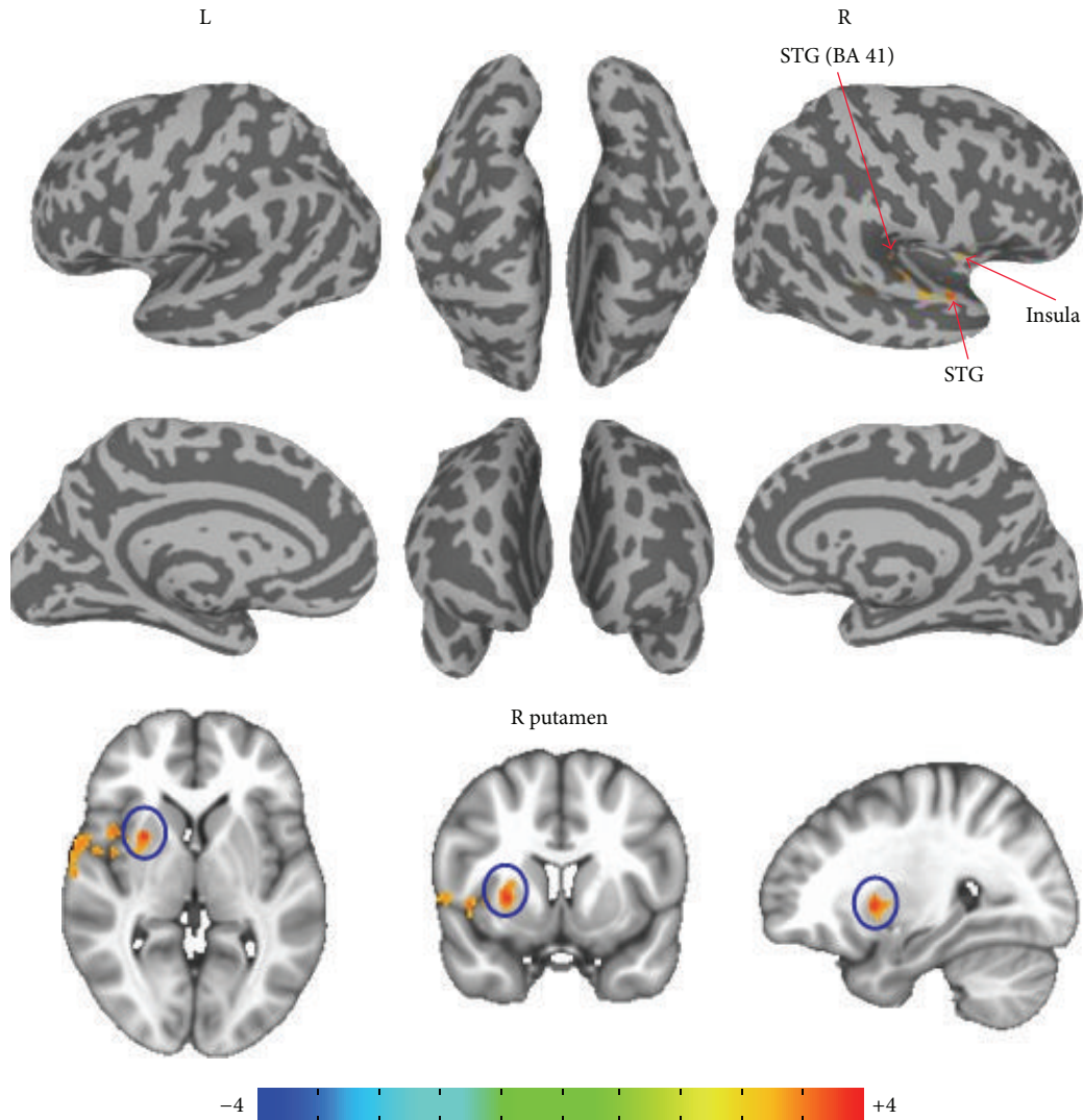
FIGURE 4: Changed functional connectivity of right ACC after acupuncture for patients with Bell's palsy at later stage. P \leq 0.01 , \alpha \leq 0.05 , corrected with Monte-Carlo method. BA: Brodmann area; STG: superior temporal gyrus; STG: superior temporal gyrus.
