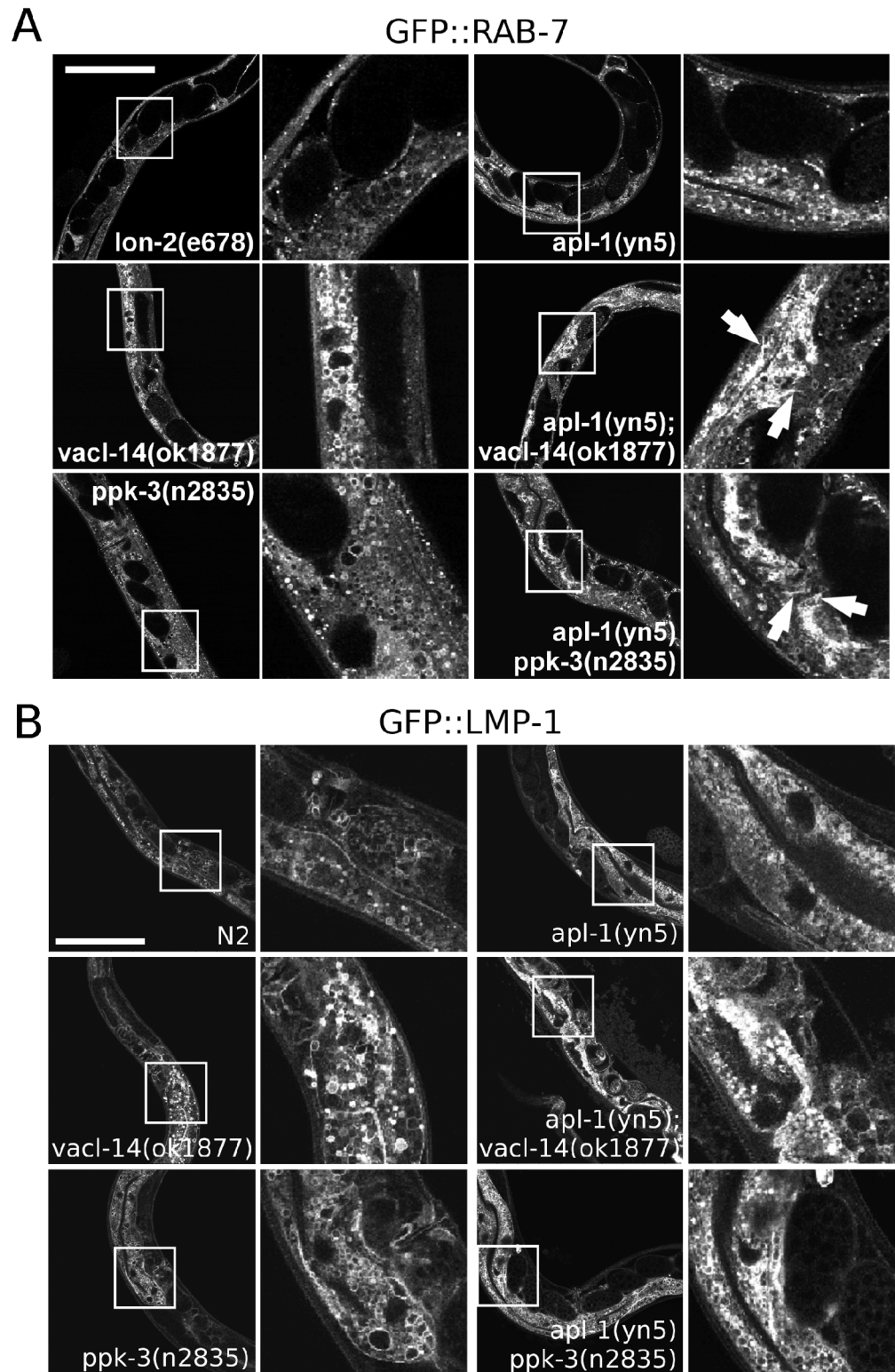
Fig 5. Mutations in apl-1 and ppk-3 or vac1-14 lead to defective processing of late endosomes and lysosomes in young adults. (A) In control animals and single apl-1(yn5) , vac1-14(ok1877) and ppk-3(n2835) mutants late endosomes stained using GFP:: RAB-7 as a marker were visible as vesicles or small vacuoles. Combination of the mutations in apl-1(yn5) ; vac1-14(ok1877) or apl-1(yn5) ppk-3(n2835) double mutants led to a drastic alteration of the morphology of the late endosomal compartment, e.g. late
