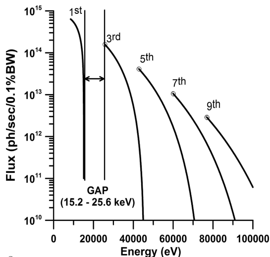
Figure 3 Flux ( \text{photons s}^{-1} 0.1\% \text{ BW}^{-1} ) as a function of energy for the undulator U23 harmonics of the undulator U23 calculated using SPECTRA 9.0.2 (Tanaka & Kitamura, 2001) at 29.3 m from the source within a 1 \text{ mm} \times 1 \text{ mm} ( 35.7 \mu\text{rad} \times 35.7 \mu\text{rad} ) aperture. This corresponds to the theoretical available flux after the second high-heat-load slit system of the beamline. In order to protect the first monochromator crystal of the HRPD beamline branch the slits are never opened larger than 1 \text{ mm} \times 1 \text{ mm} . The calculated flux values are used as a starting value for the ray-tracing calculation in SHADOW after the first high-heat-load slit system. The energy spectrum of U23 has a gap between 15.2 keV of the first and 25.6 keV of the third harmonic (minimum gap of 10 mm). Fixed energies of 25.6, 42.7, 60.0 and 77.1 keV used at the beamline are highlighted by the open circles at the end of the third, fifth, seventh and ninth harmonic and correspond to maximum flux reachable at the minimum gap of \sim 10 \text{ mm} .
