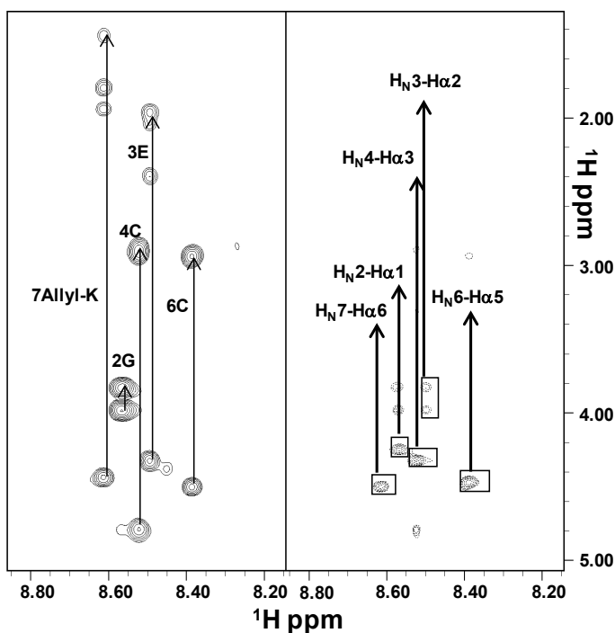
Figure 3. Comparison of 2D [ ^1\text{H} , ^1\text{H} ] TOCSY ( left ) and ROESY 200 ( right ) spectra of PepK in \text{H}_2\text{O}/\text{D}_2\text{O} (90/10). The two sides of the figure show spectral regions containing \text{H}_\text{N} /aliphatic protons correlations; spin system assignments are indicated in the TOCSY left panel. In the right panel, sequential ROE contacts are shown.
