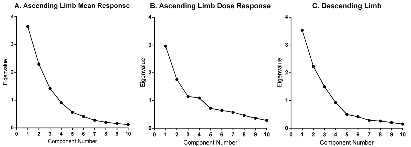
Figure 1. Scree plots of subjective responses to alcohol in the full sample in terms of (A) ascending limb mean response across the alcohol challenge, (B) change in response along an ascending limb alcohol dose, and (C) descending limb of the alcohol challenge.
