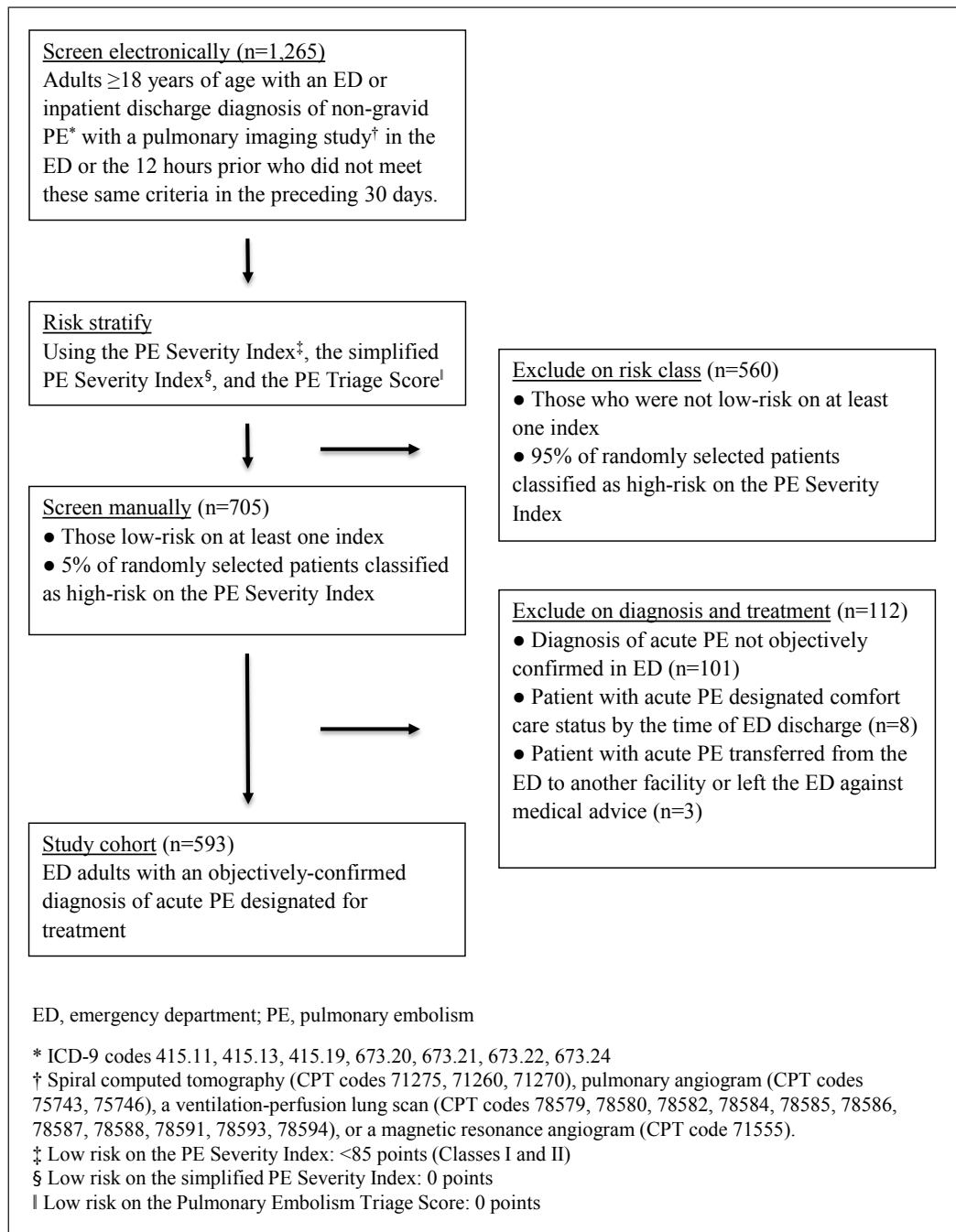
Fig. 1 Cohort assembly
