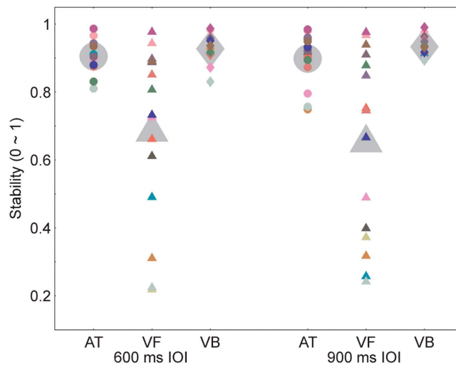
Figure 2. Results of experiment 1. Tapping was most stable for the visual bouncing ball sequence. The mean synchronization stabilities are indicated by the large gray marks. The data from individual subjects are indicated by the small marks of different colors, which indicate different subjects. AT, VF and VB represent the auditory tone sequence, visual flashing ball sequence, and visual bouncing ball sequence, respectively.
