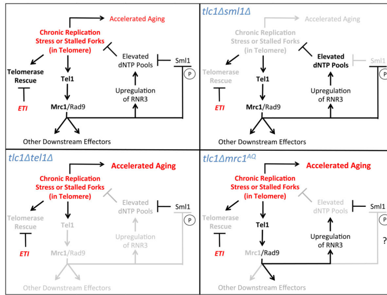
Figure 7. Proposed Model
