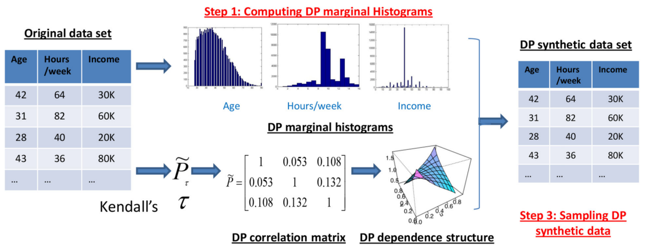
Step 2: Computing DP correlation matrix through DP Kendall's tau
