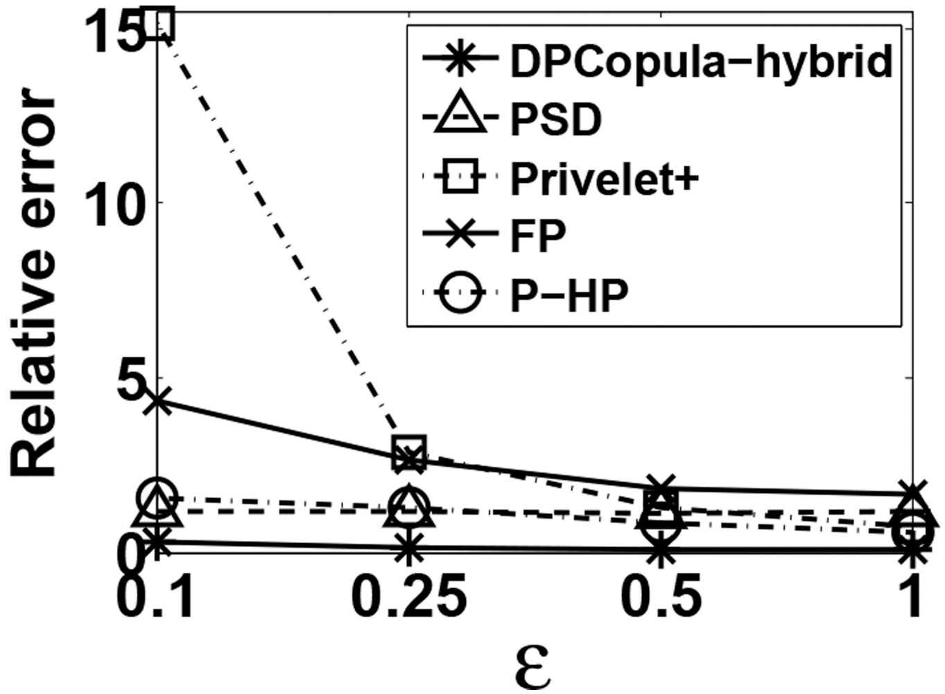
Figure 4. Comparison with other methods
