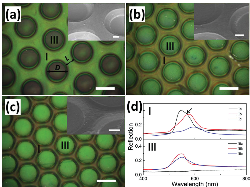
Figure 4. (a–c) Optical images of imprinted micropatterns on POFs with stamps of different post separation, L = 80, 50, 30 \mu\text{m} . Scale bars are 100 \mu\text{m} and 20 \mu\text{m} in insets. (d) Reflection spectra of patterns in (a–c) within regions I and III. Arrow indicates shoulder peak.
