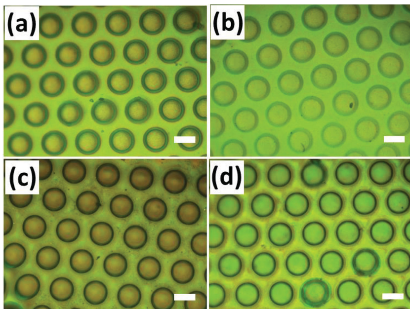
Figure 5. Optical images of adjustable structural color patterns under different imprinting conditions. (a) 110 °C, 10 bar, 150 s, (b) 90 °C, 30 bar, 150 s, (c) 110 °C 50 bar, 150 s, (d) 110 °C, 30 bar, 60 s. All of them have the same gap width of 80 \mu\text{m} as in Figure 4a. All scale bars are 100 \mu\text{m} .
