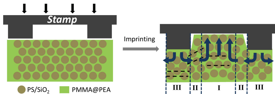
Scheme 1. Mechanism of pattern formation by microimprinting in POFs. Region I is the extruded region, region II is the transition region, and region III is the imprinted region.
