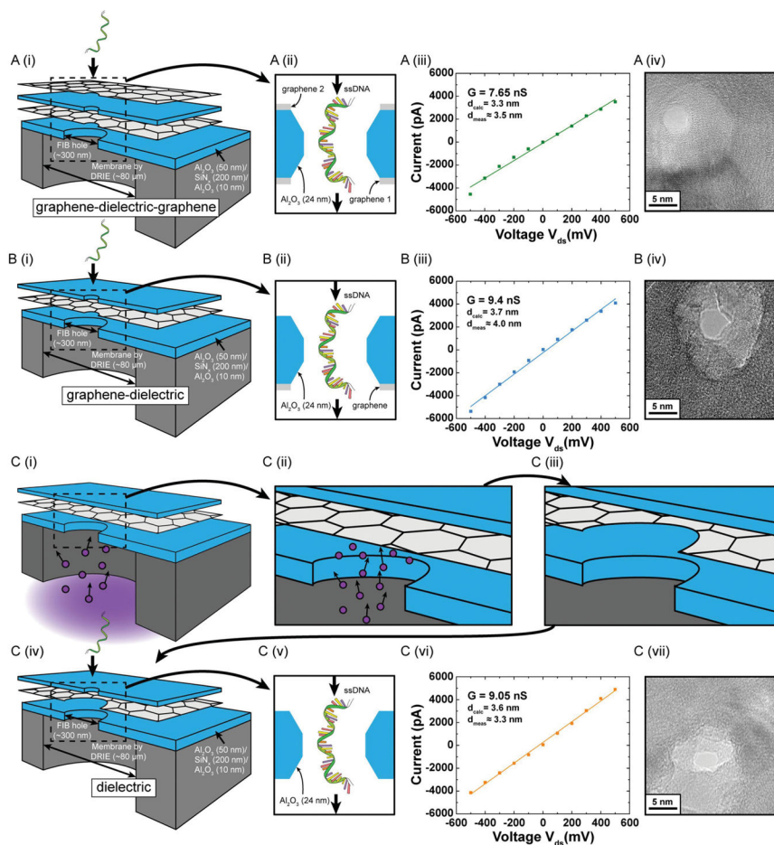
Figure 1. Schematic of the membrane structures whose DNA interaction and translocation properties are compared in this study. A) (i) Sequential transfer of graphene followed by atomic layer deposition (ALD) of 24 nm \text{Al}_2\text{O}_3 is followed by another graphene layer transfer. (ii) The nanopore region is magnified and dimensions of the dielectric layer are indicated. (iii) IV curve for an \approx 3.5 nm pore in a graphene–dielectric–graphene membrane. (iv) TEM image of the nanopore. B) (i) Graphene transfer was followed by ALD deposition of \text{Al}_2\text{O}_3 . (ii) The nanopore region is magnified. (iii) Open pore IV curve for an \approx 4 nm pore in a graphene–dielectric membrane. (iv) TEM image of the nanopore. C) [(i)–(iv)] Graphene transfer was followed by ALD deposition of \text{Al}_2\text{O}_3 . Reactive ion etching in an oxygen plasma environment is then used to etch the exposed graphene leaving only the oxide layer. (v) The nanopore region is magnified. (vi) Open pore IV curve for an \approx 3.3 nm pore in a dielectric membrane. (vii) TEM image of nanopore. The nanopore diameters (scale bar 5 nm) are comparable and the ionic conductivity is almost similar in all three cases, essential for direct comparison of DNA translocation properties. All experiments were done in 1 M KCl, 10 \times 10^{-3} M Tris, 1 \times 10^{-3} M EDTA at pH 7.6. 100nt ssDNA is threaded from source to drain as indicated for all the cases studied here.
