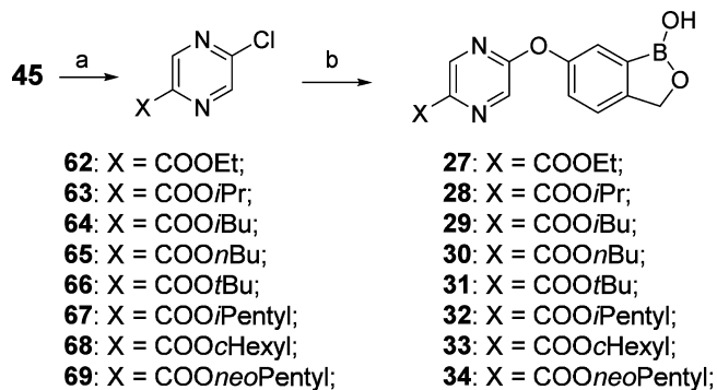
Scheme 8. Syntheses of Ester Compounds 27–34 a
