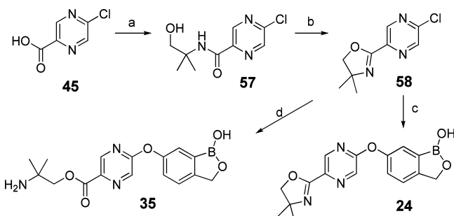
Scheme 6. Synthesis of Compounds 24 and 35 a
