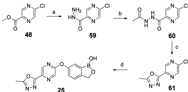
Scheme 7. Synthesis of Compound 25 a
