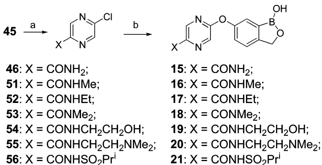
Scheme 5. Synthesis of Compounds 15–21 a
