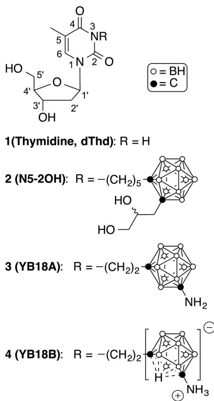
Fig. 1. Structures of 1 , the first generation 3CTA 2 , and the second generation 3CTAs 3 and 4 .
