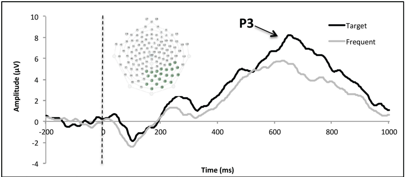
Figure 1. P3 electrode cluster and P3 waveforms for target and frequent trials. The waveform depicted represents the mean waveform from those electrodes with a 0.4 or greater factor loading onto the PCA component reflecting the P3; electrodes were averaged with equal, unit weighting. The P3 amplitudes in Table 1 were calculated from PCA. In the PCA, all electrodes contribute to the estimation of amplitudes to the extent that they reflect the underlying P3 component (based on factor loadings), thus accentuating those electrodes that are driving the signal. This accounts for the larger amplitudes in Table 1 than Figure 1.
