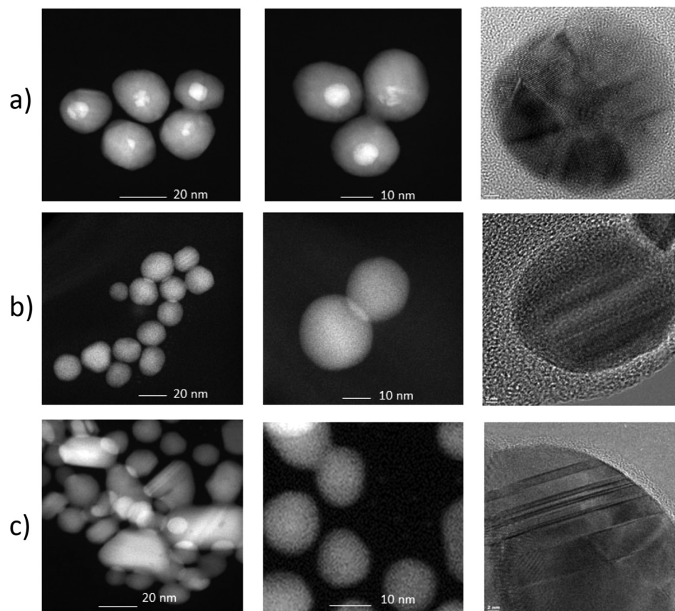
FIG. 1. Representative HAADF STEM (columns 1 and 2) and HR-TEM (column 3) images of the (a) \text{Ag}^{\text{Au}}_{20}\text{NPs} , (b) \text{Ag}^{\text{pn}}_{20}\text{NPs} , and (c) \text{Ag}^{\text{pi}}_{20}\text{NPs} stock particles.
