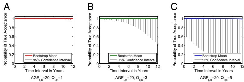
Fig. 3. Population-mean trend and 95% confidence interval of probability of true acceptance ( \pi_{ijk} ) with respect to \Delta T_{ijk} when AGE_{ijk} is 20 and Q_{ijk} is (A) 1, (B) 3, and (C) 5 in model D*. The decision threshold is set to the value corresponding to FAR of 0.00001%. Match scores are obtained by COTS-1 matcher when a single finger is used for recognition.
