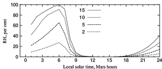
Figure 14. Simulated relative humidity values at 1 m altitude for the MSL landing site using an atmospheric column model [Savijärvi et al. , 2004]. The simulation assumed water being initially uniformly mixed in the atmosphere with absolute precipitable water contents of 2, 5, 10, and 15 pr \mu\text{m} .
