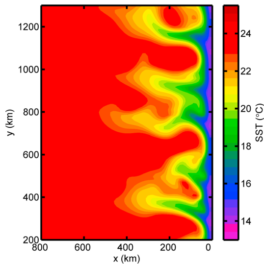
Figure 2. Model snapshot (5 days average) of simulated sea surface temperature ( ^{\circ}\text{C} ) in January shows mesoscale eddy activities of the Chilean upwelling system. As in the model, data from hydrographic stations, satellite observation, and other model studies show a relatively uniform inner coast-parallel zone of \sim 50 km wide with 15 - 19^{\circ}\text{C} upwelled waters and \sim 100 km radius of mesoscale activities [Blanco et al. , 2001; Thomas et al. , 2001; Chaigneau et al. , 2009; Colas et al. , 2011].
