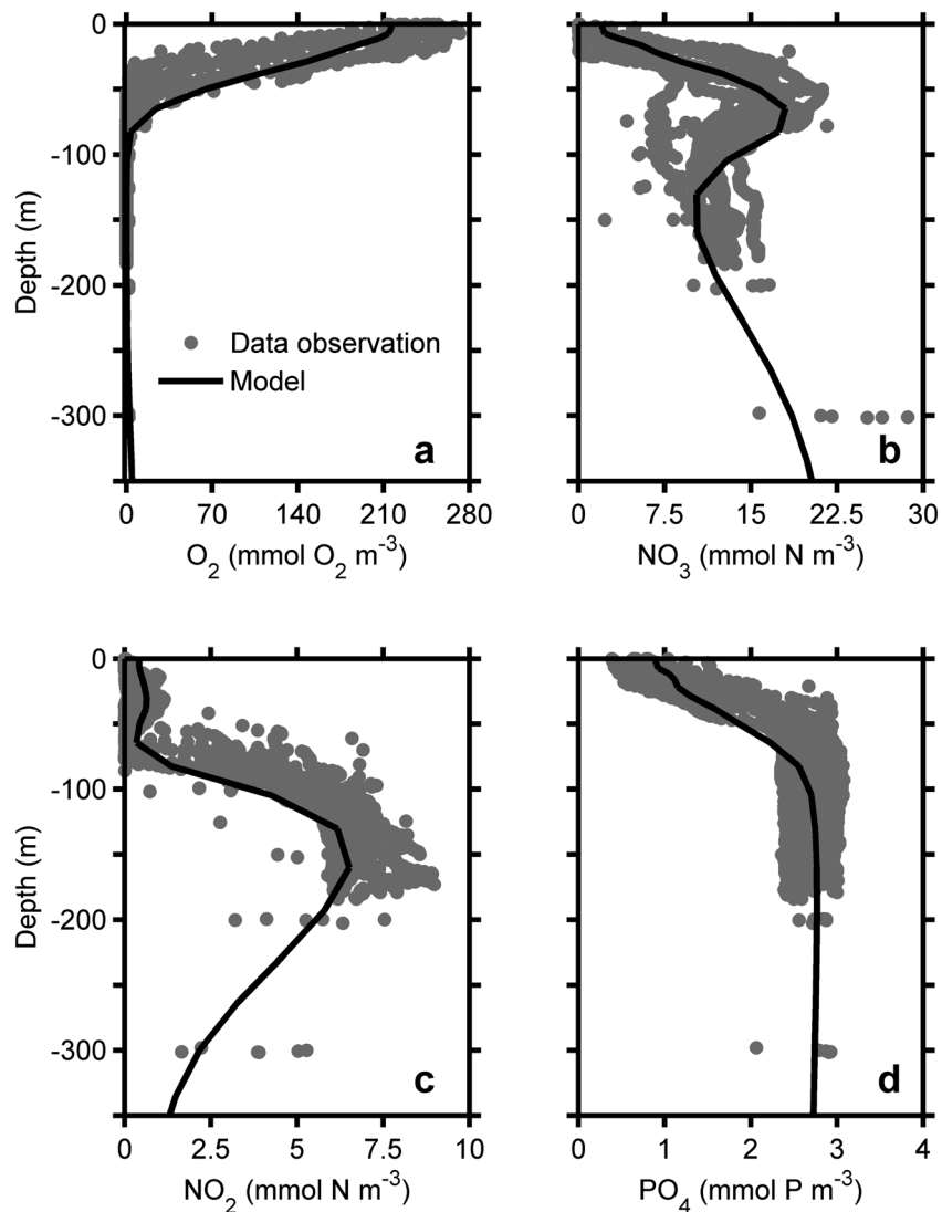
Figure 4. Modeled and observed (a) oxygen, (b) nitrate, (c) nitrite, and (d) phosphate concentration offshore Chile (~ 20°S). The solid black lines are the modeled results. The grey circles represent station data from 2009 and 2010 cruises. The results are averaged over January in the last two years of the simulation, alongshore, and from the coast to 80 km offshore. Note the reduced nitrate concentration and presence of the nitrite maximum in the oxygen-minimum depth of 100 to 200 m.
