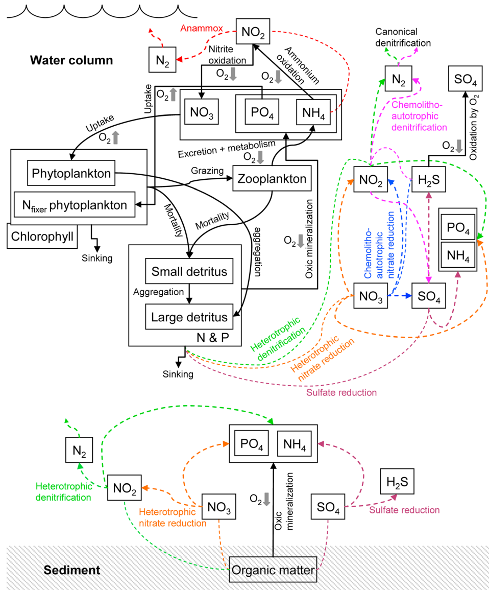
Figure 1. Flow diagram of the ecosystem-biogeochimical model. The model consists of 14 state variables (see Appendixes for detail). Anaerobic processes of remineralization and oxidation are highlighted by dashed lines. Processes which produce (consume) oxygen are indicated by up (down) gray thick arrows. It is worth to note that canonical denitrification is the sum of heterotrophic denitrification and sulfide-driven denitrification. Organic matter that reaches the seafloor is assumed to be remineralized instantaneously by oxic and/or anoxic remineralizations.
