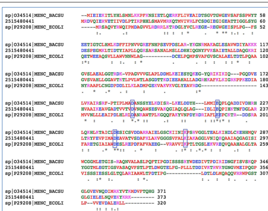
Figure 3 Multiple sequence alignment of MenC from E. coli , B. subtilis and predicted MenC in P. roseus (IMG 2515480441) showing conserved amino acids predicted to be essential for proper functioning of the enzyme.
