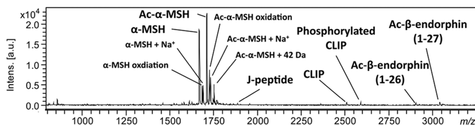
Figure 2. Mass spectrum acquired from a melanotroph. Several peptides from the POMC prohormone are detected, including \alpha -MSH, joining peptide (J-peptide), corticotropin-like intermediate peptide (CLIP), and \beta -endorphin.
