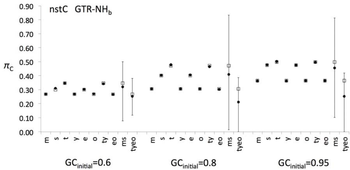
Figure S1. Actual and estimated equilibrium frequencies of nucleotide C ( \pi_C ) at nodes on the tree for selection scheme nstC under (A) the GTR-NH and (B) the GTR-NH b models. Three initial GC biases (with GC_{\text{initial}} = 0.6, 0.8 and 0.95 ) were considered. Shown are the averages and 95% confidence intervals over 300 bootstrap replicate datasets generated by bootstrap resampling of the 777,600 sites in the simulated dataset. Note that the results for the two branches around the root (ms and tyeo) are highly unreliable.
