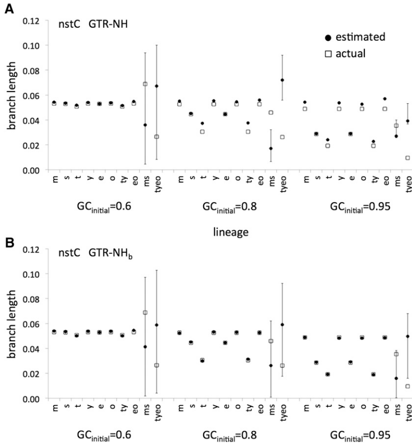
Figure 6 (A and B) Actual and estimated branch lengths under the GTR-NH (A) and GTR-NH b (B) models for data simulated under the nstC scheme. Three GC initial levels (0.6, 0.8, and 0.95) are used. Actual branch length was calculated as the observed number of substitutions on the branch divided by the number of sites. Estimated branch length was calculated as the expected number of substitutions per site when the base compositions are in equilibrium for the substitution rate matrix (Yang and Roberts 1995), but the new definition of Equation 7 gave similar values. The two branch lengths around the root of the tree should be ignored. Shown are the averages and 95% confidence intervals over 300 bootstrap replicate data sets, generated by bootstrap resampling of the 777,600 sites in the simulated data set.
