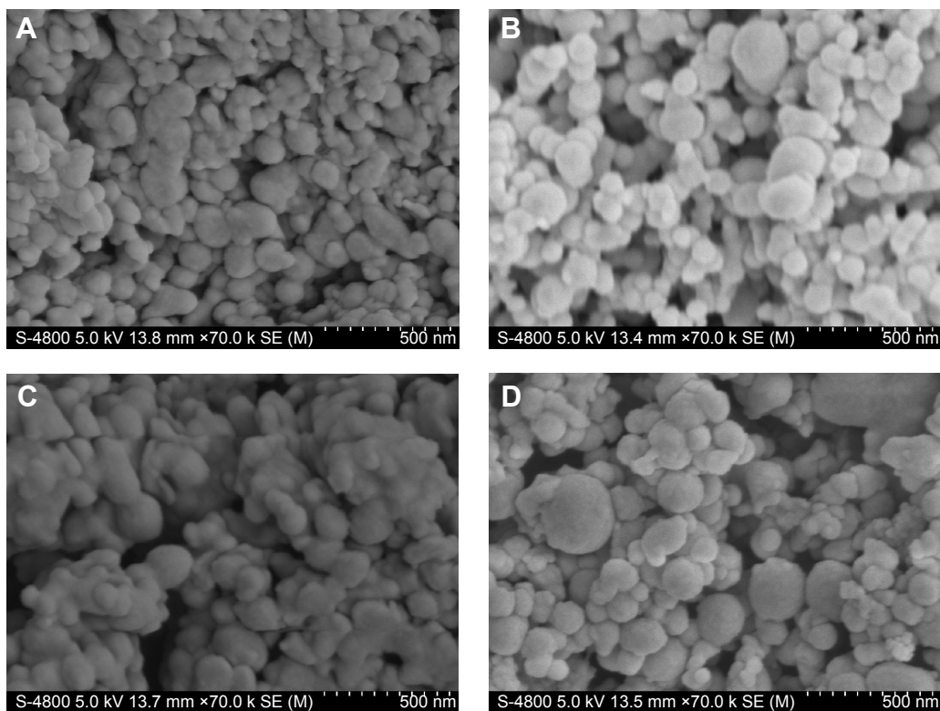
Figure S1 SEM photographs of \text{Fe}_3\text{O}_4 -SF nanoparticles in different ratios of SF/ \text{Fe}_3\text{O}_4 .
