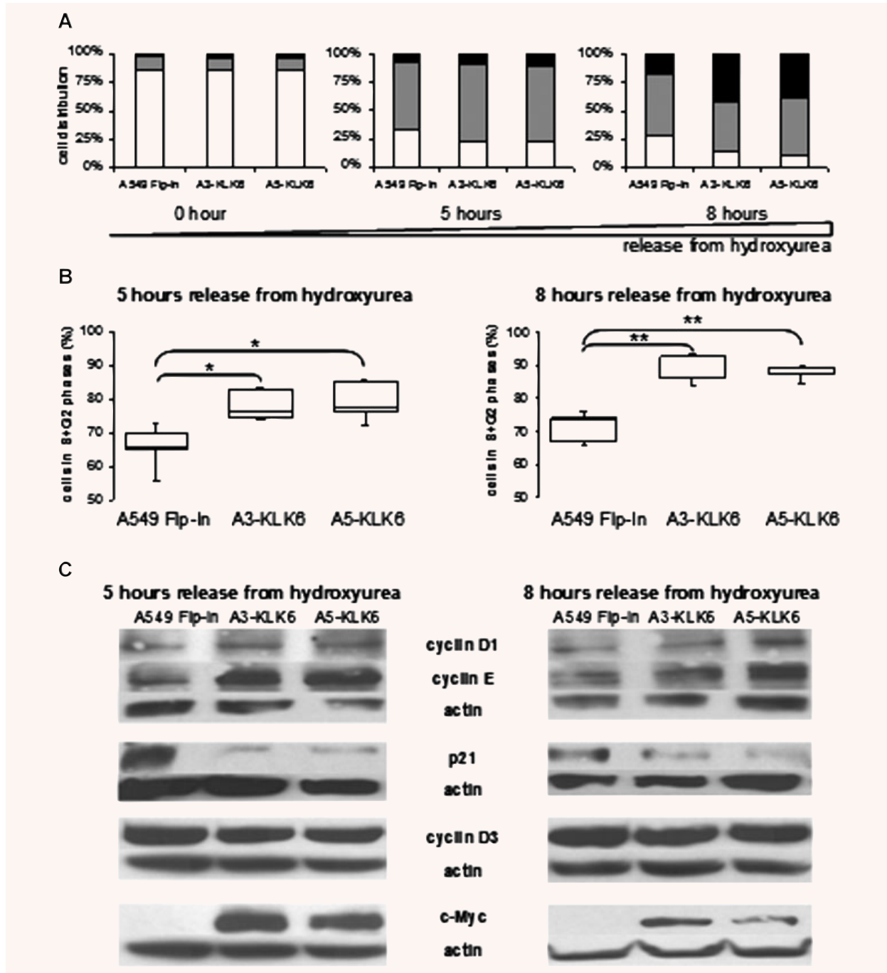
Fig. 3 Effect of KLK6 on NSCLC cell growth and regulation of cell cycle progression. (A) Distribution of control A549 Flp-In and A3-KLK6 and A5-KLK6 cells within the G1 (white), S (grey) and G2 (black) phases of the cell cycle 0, 5 or 8 hrs after release from hydroxyurea. Results are expressed as the median values of five independent experiments. (B) Box plot of control A549 Flp-In and A3-KLK6 and A5-KLK6 cells passed from G1 into G2+S phases 5 and 8 hrs after release from hydroxyurea. Results are representative of five independent experiments. P -values were determined using a Kruskal and Wallis test. * P < 0.05, ** P < 0.025. (C) Assay of cell-cycle proteins and c-Myc by Western blotting of whole-cell extracts (50 μg) from the control A549 Flp-In, A3-KLK6 and A5-KLK6 lines 5 and 8 hrs after release from hydroxyurea. Actin protein was used to check for equal loading. Results are from one of three experiments.
