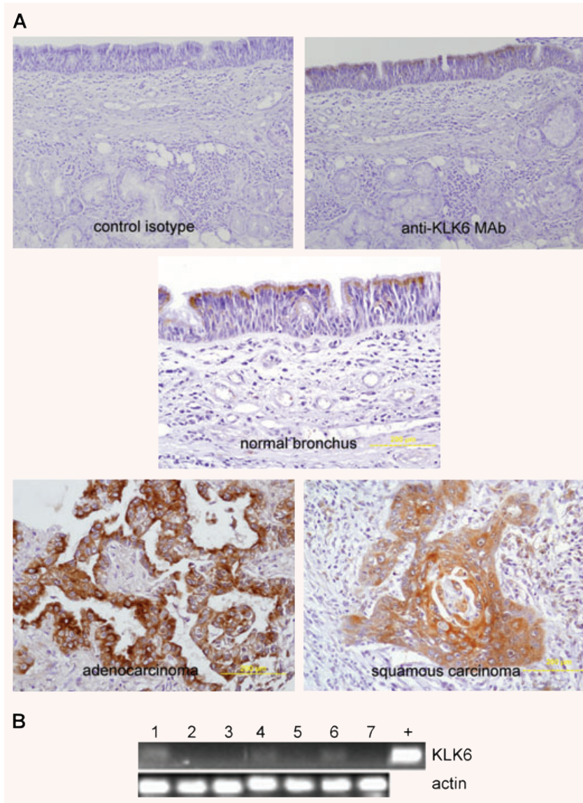
Fig. 1 KLK6 in tissues from patients with NSCLC but not in NSCLC-derived cell lines. (A) Immunohistochemistry of KLK6 in normal and malignant lung from 46 patients with primary NSCLC using a monoclonal antibody (original magnification: \times 200 ; haematoxylin counterstain). KLK6 immunostaining (dark) in the apical region of normal bronchial epithelial cells (thin arrow) and in the cytoplasm of most cancer cells (large arrow). (B) KLK6 production in a panel of NSCLC lines by RT-PCR. Total RNA from NSCLC cell lines was extracted and reverse transcribed. KLK6 and \beta -actin (internal control) mRNAs were amplified from cDNA by PCR and the amplification products were separated on a 1% agarose gel containing ethidium bromide. (1) A549; (2) Calu-1; (3) H23; (4) H460; (5) H520; (6) H522; (7) H1838; +: plasmid containing KLK6 cDNA.
