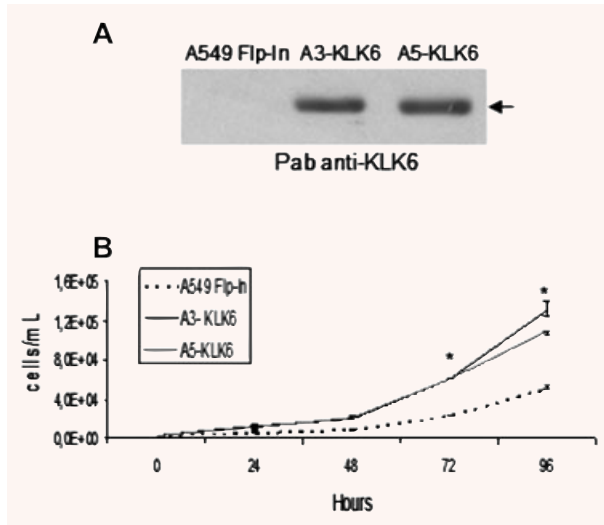
Fig. 2 Ectopic KLK6 in NSCLC promotes proliferation. (A) Secretion of KLK6 by A549 Flp-In and stable isogenic clones (A3- and A5-KLK6) assessed by Western blotting using a polyclonal anti-KLK6 antibody. Equal volumes of cell culture supernatant were loaded onto 12% SDS-PAGE gels. (B) Control A549 Flp-In (dashed line) and A3-KLK6 (black full line) and A5-KLK6 (grey full line) ( 2.5 \times 10^3 cells of each) were seeded and cells were counted at the indicated times. Points, median value of triplicate determinations from one representative experiment (of three). Bars, lower and upper quartiles. P -values were determined using a Kruskal and Wallis test. * P < 0.05.
