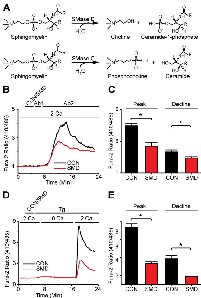
Figure 1. SMase D suppresses SOCE in human T lymphocytes. (A) Reaction schemes for SMase D (top) and SMase C (bottom). (B) Fura-2 ratio signals of (26–54) T cells in a single 40 \times field, where the records show the average signals relative to the resting levels. The upper bar above the panel indicates these treatments: after 2-min rest, cells were treated with either SMase D (SMD, red) or catalytically inactive enzyme (CON, black) for 3 min, and then with 5 \mu\text{g} anti-CD3 \epsilon (Ab1) antibody for 2 min, and finally with 5 \mu\text{g} anti-IgG (Ab2) antibody for 18 min; the lower bar shows the \text{Ca}^{2+} -containing solution type. (C) Peak and declining phase (at 23 min) values (error bars represent mean \pm SEM; n = 5 ) of Fura-2 ratio signals after antibody stimulation as shown in B. (D) Fura-2 ratio signals of (17–31) T cells as in B, where the upper bar above the panel refers to these treatments: after 2-min rest, cells were treated with SMD (red) or CON (black) for 3 min and 1 \mu\text{g} Tg for 18 min; the lower bar shows the \text{Ca}^{2+} -containing solution type. (E) Peak and declining phase (23 min) values (error bars represent mean \pm SEM; n = 5 ) of Fura-2 ratio signals from Tg-stimulated cells for experiments as shown in D. Where present, the asterisks denote statistically significant comparisons as detailed in Materials and methods.
