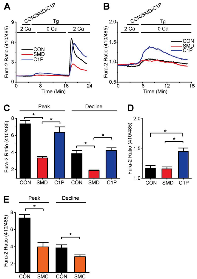
Figure 4. T lymphocyte SOCE is inhibited by SMases but not CIP. (A) Fura-2 ratio signals of (35–45) T cells, where the upper bar above the panel indicates treatments: after 2-min rest, cells were treated with SMase D (SMD, red), C1P (blue), or catalytically inactive enzyme (CON, black) for 3 min and 1 \mu\text{g} Tg for 18 min; the lower bar shows the \text{Ca}^{2+} -containing solution type. Cells treated with C1P were also bathed in 0.5 mg/ml of CIP-containing solutions throughout the Tg treatment period. (B) Fura-2 ratio signals from experiments shown in A but with axes rescaled to better show the internal store release component for cells treated with SMD (red), C1P (blue), or CON (black). (C) Peak and declining phase (23 min) values (error bars represent mean \pm SEM; n = 5 ) of Fura-2 ratio signals from Tg-stimulated cells for experiments as shown in A. (D) Peak values (error bars represent mean \pm SEM; n = 5 ) of Fura-2 ratio signals from Tg-stimulated cells in experiments as shown in B. (E) Peak and declining phase values (error bars show mean \pm SEM; n = 5 ) of Fura-2 ratio signals from Tg-stimulated cells treated with SMase C (SMC, orange) or CON (black). Where present, the asterisks denote statistically significant comparisons as detailed in Materials and methods.
