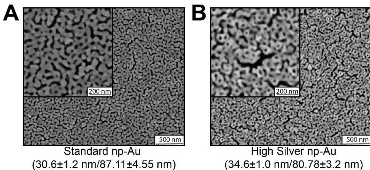
Figure 2. (A) Scanning electron micrographs of the standard (4% silver) np-Au surface and (B) the high-silver content (12% silver) np-Au surface. The low-magnification SEM micrographs demonstrate the long-range uniformity of our np-Au substrate. High magnification (100 kX) micrographs are shown in the insets, and measured ligament lengths and pore diameters are shown below.
