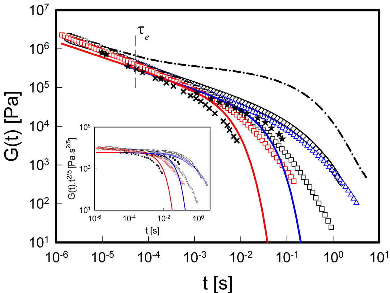
Figure 2. Stress relaxation modulus for PI rings and PS rings at T-T_g=65^\circ\text{C} . PI 81k ( \blacktriangle ); PI 38k ( \square ); PS198k ( \blacklozenge ); PS160k ( \square ). The stars and the crosses are from molecular dynamic simulations on coarse grained bead-spring rings with Z\approx 3.6 and 14.4 from Ref. (24) (see Supplementary Information for details about the conversion of MD units into Pascal and seconds). The blue and the red lines are model prediction for PI 81k and 38k, respectively. The dash-dotted line is the relaxation modulus for PI 81k linear polymer, exhibiting an entanglement plateau. The Rouse time for entanglements \tau_e , of the linear PI81k is also depicted for reference. Inset: Scaled version of the same plot, without the linear polymer data for clarity (see text for details).]
