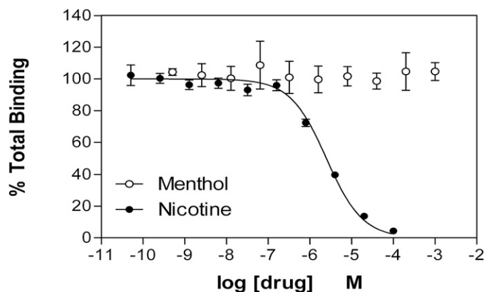
Fig. 2. Menthol does not compete for the nAChR agonist binding site labeled by [^3H] epibatidine. Membranes from human embryonic kidney cells expressing \alpha 3\beta 4 nAChRs were incubated for 2 hours with \sim 0.5 nM [^3H]EB in the absence or presence of increasing concentrations of menthol or nicotine. The membranes were then filtered and counted. Data were analyzed by nonlinear least-squares regression analysis. The K_i of nicotine in these studies was 256 nM. Menthol at concentrations up to 1 mM did not compete for these receptors. Data shown are the mean \pm S.E.M. of five independent assays.
