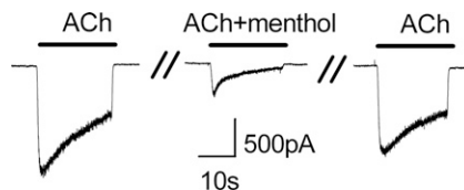
Fig. 9. Menthol inhibits ACh-evoked currents in nodose ganglia neurons. Representative current traces in a voltage-clamped neuron evoked by ACh ( 30 \mu\text{M} ) and ACh plus menthol ( 100 \mu\text{M} ). Note that menthol increases the speed and extent of desensitization. The cell was washed for 60 seconds between ACh applications.
