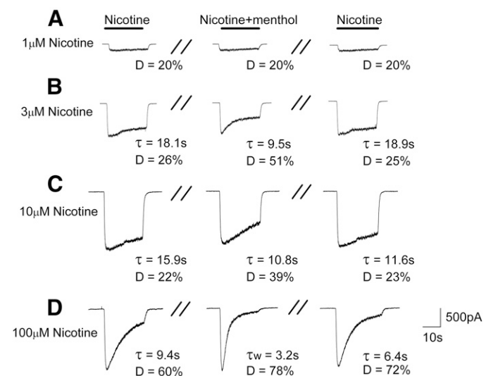
Fig. 7. Menthol enhances the desensitization of the currents evoked by nicotine. Representative inward currents induced by (A) 1 \mu\text{M} , (B) 3 \mu\text{M} , (C) 10 \mu\text{M} , and (D) 100 \mu\text{M} nicotine in the absence of menthol (left), presence of 100 \mu\text{M} menthol (middle), and 5 minutes after washout of the menthol (right). Time constant ( \tau ) and the extent of desensitization (D) were used to characterize the desensitization.
