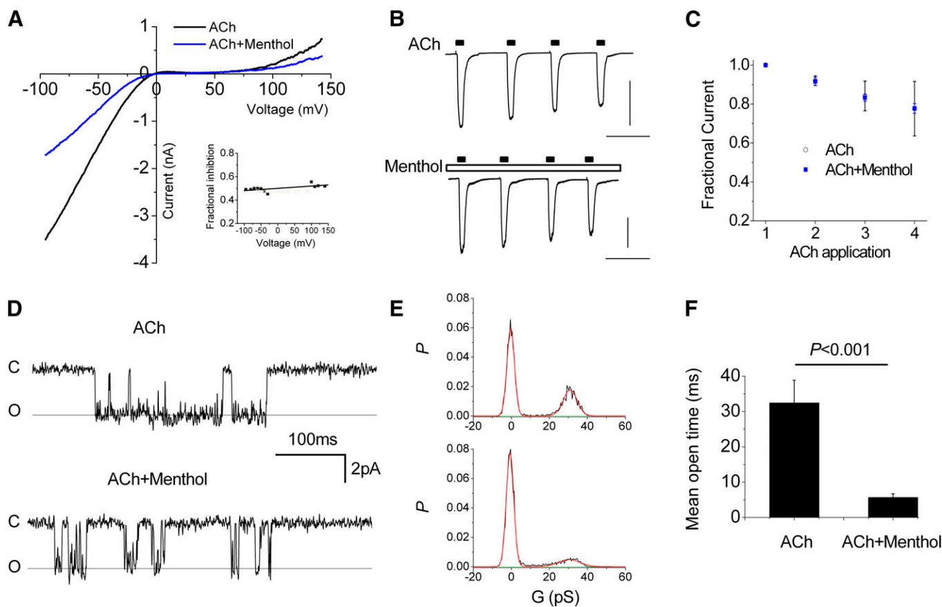
Fig. 5. Menthol inhibits \alpha 3\beta 4 nAChRs in a voltage- and use-independent manner and without affecting single-channel conductance. (A) Current-voltage relationship for peak response to ACh (30 \mu M) and after 20-second application of menthol (100 \mu M). The background current in the absence of ACh is subtracted. The inset shows the fraction of the menthol versus control current at indicated potentials. (B) Responses to repeated, 5-second stimulation with ACh (30 \mu M) under control conditions (upper trace) or in the presence of 200 \mu M menthol (lower trace). Scale bars, 1 nA and 20 seconds. (C) Mean peak responses to ACh from experiments depicted in (B) ( n = 3 ). (D) Representative single-channel currents from a cell-attached patch ( V_M, -110 mV, 10 \mu M ACh in pipette) under control conditions (upper trace) and in the presence of 200 \mu M menthol. (E) All-points histograms constructed from 2 seconds of continuous data. The smooth lines represent best-fits to Gaussian functions yielding similar conductances (G) of 30.9 and 30.3 pS respectively. (F) Mean open time measured from data in (E) (measured from >50 events).
