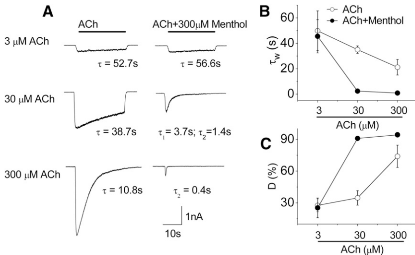
Fig. 4. Menthol modulation of \alpha 3\beta 4 nAChRs is dependent on the concentration of ACh. (A) Representative whole-cell inward currents in response to different concentrations of ACh in the absence (left) and in the presence (right) of 300 \mu\text{M} menthol in \alpha 3\beta 4 nAChR-expressing cells. The current decay during desensitization was best fit to a one- or two-exponential function, yielding the indicated time constants. (B) Mean weighted average time constants for decay and (C) percent of desensitization (D) of the ACh-mediated current obtained in the absence of menthol (open circle) and in the presence of 300 \mu\text{M} of menthol (filled circle). Data are mean \pm S.E.M., n = 3-5 .
