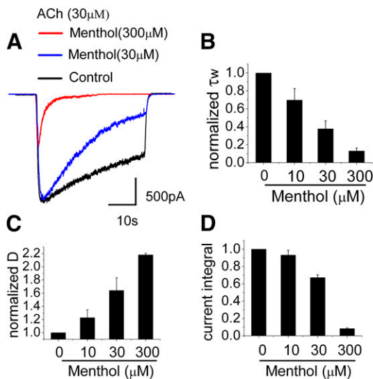
Fig. 6. Concentration-dependent effects of menthol. (A) Representative currents activated by ACh (30 \mu\text{M} ) and ACh plus menthol (30 and 300 \mu\text{M} ); (B) Bar graph of time constant; (C) the fraction of desensitized (D) receptors; and (D) the current integrals in response to the concentration of menthol from 10 to 300 \mu\text{M} , which was coapplied with 30 \mu\text{M} ACh. Data are the normalized means \pm S.E.M. of three to six experiments.
