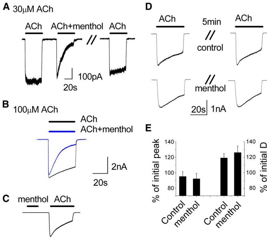
Fig. 3. Menthol enhances the decay of ACh-evoked currents. Representative inward currents in HEK293 cells expressing \alpha 3\beta 4 nAChRs in response to (A) 30 \mu\text{M} ACh and (B) 100 \mu\text{M} , with or without menthol (100 \mu\text{M} ) and after 60-second washout (A). The holding potential was -50 mV. (C) Menthol (100 \mu\text{M} ) alone evokes no current. (D) A 5-minute pretreatment with menthol (100 \mu\text{M} ) alone does not affect the subsequent current evoked by ACh (30 \mu\text{M} ). (E) Summary of the peak current evoked by ACh and amount of current decay following 5-minute pretreatment with either control or menthol ( n = 3 ). D, desensitization.
