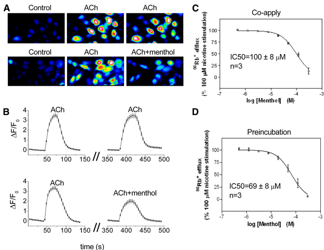
Fig. 1. Effects of menthol on human \alpha 3\beta 4 nAChR-mediated [Ca^{2+}] influx and nicotine-stimulated ^{86}Rb^{+} efflux. (A) Representative Fluo-4 fluorescence images of \alpha 3\beta 4 -expressing HEK293 cells captured during control, repeated application of 30 \mu M ACh (upper images), or application of 30 \mu M ACh alone and ACh plus 100 \mu M menthol (lower images). (B, upper trace) Mean Fluo-4 fluorescence during repeated application of ACh ( n = 39 cells) or (B, lower trace) ACh and ACh plus menthol ( n = 37 cells). The interstimulus interval was 5 minutes. (C) Inhibition of nicotine-stimulated ^{86}Rb^{+} efflux in the presence of menthol or (D) 10-minute preincubation with menthol; n = 3 independent assays.
