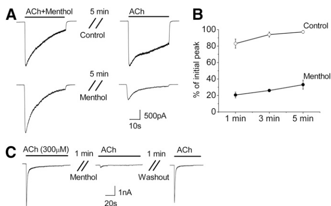
Fig. 8. Menthol hinders the recovery of \alpha 3\beta 4 nAChRs from desensitization. (A) Representative inward currents showing desensitization induced by coapplied 30 \mu\text{M} ACh and 100 \mu\text{M} menthol and the subsequent response to ACh following a 5-minute wash in either the control bath solution (upper traces) or 100 \mu\text{M} menthol (lower traces). (B) Time course for recovery following the treatment described in (A), control (open circles), and menthol (closed circles). Data are the means \pm S.E.M. of three to five experiments. (C) Menthol ( 100 \mu\text{M} ) prevents recovery of \alpha 3\beta 4 nAChRs following desensitization with 300 \mu\text{M} ACh, but receptors almost fully recover after 1 minute washout with control solution ( n = 3 ).
